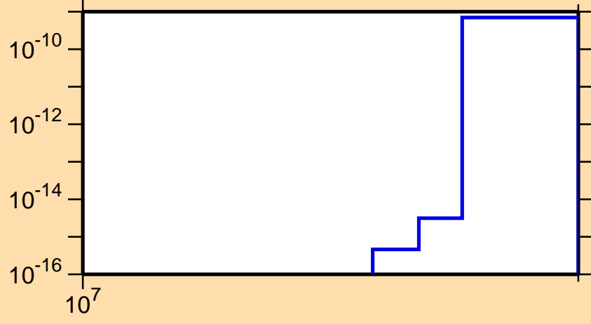
\sigma vs. E for ^{70}\text{Ge}(n,2n\alpha)
