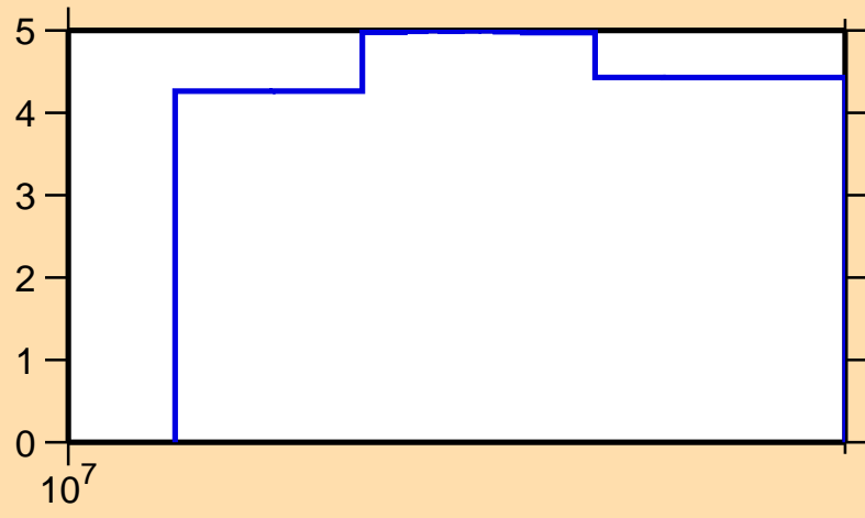
\Delta\sigma/\sigma vs. E for ^{70}\text{Ge}(n,\text{el.})
