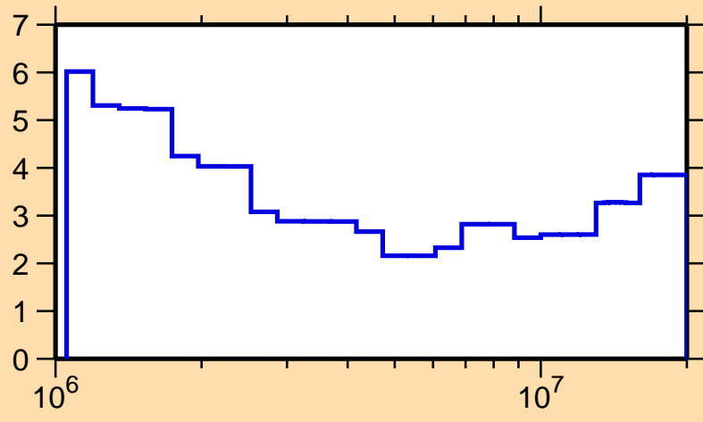
\Delta\sigma/\sigma vs. E for ^{70}\text{Ge}(n,\text{inel.})
