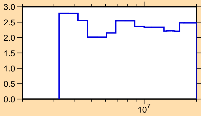
\Delta\sigma/\sigma vs. E for ^{70}\text{Ge}(n,n\text{onel.})
