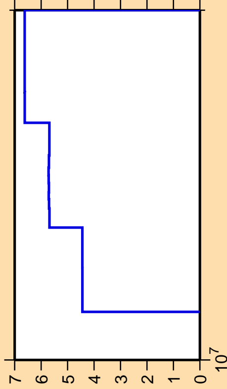
\Delta\sigma/\sigma vs. E for ^{70}\text{Ge}(n,n\text{cont.})
