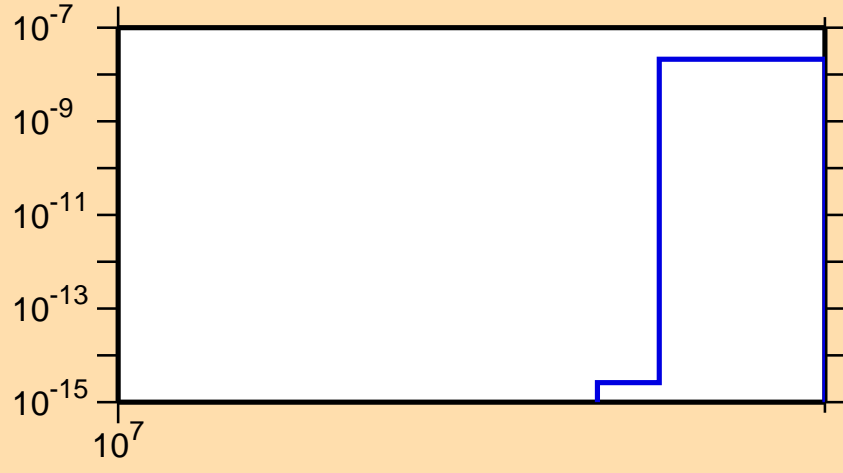
\sigma vs. E for ^{70}\text{Ge}(n,\text{nd})
