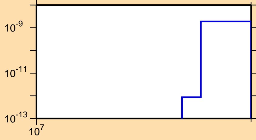
\sigma vs. E for ^{70}\text{Ge} (mt117)
