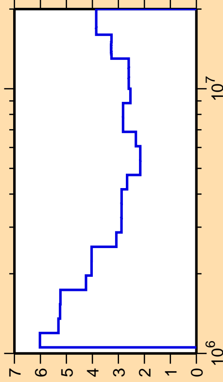
\Delta\sigma/\sigma vs. E for ^{70}\text{Ge}(n,\text{inel.})
