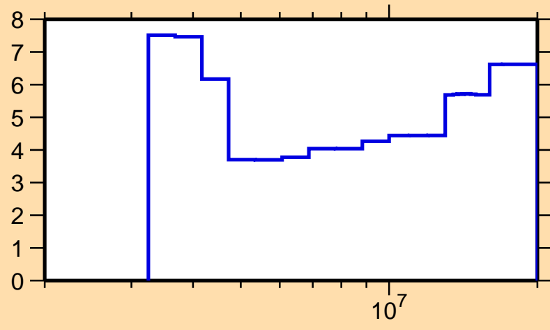
\Delta\sigma/\sigma vs. E for ^{70}\text{Ge}(n,n\text{cont.})
