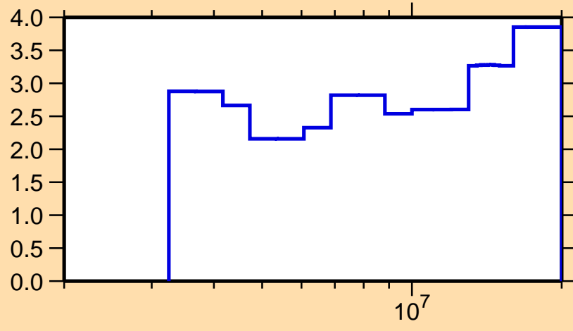
\Delta\sigma/\sigma vs. E for ^{70}\text{Ge}(n,\text{inel.})
