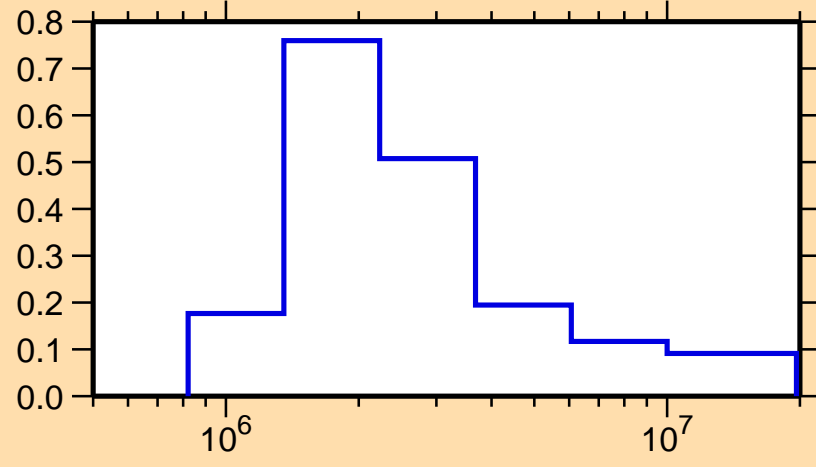
\sigma vs. E for ^{70}\text{Ge}(n,n_1)
