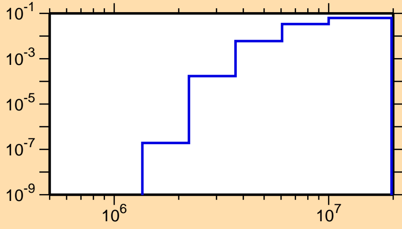
\sigma vs. E for ^{70}\text{Ge}(n,p)
