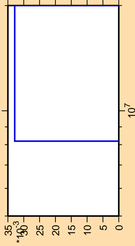
\Delta\sigma/\sigma vs. E for ^{70}\text{Ge} (mt 45)
