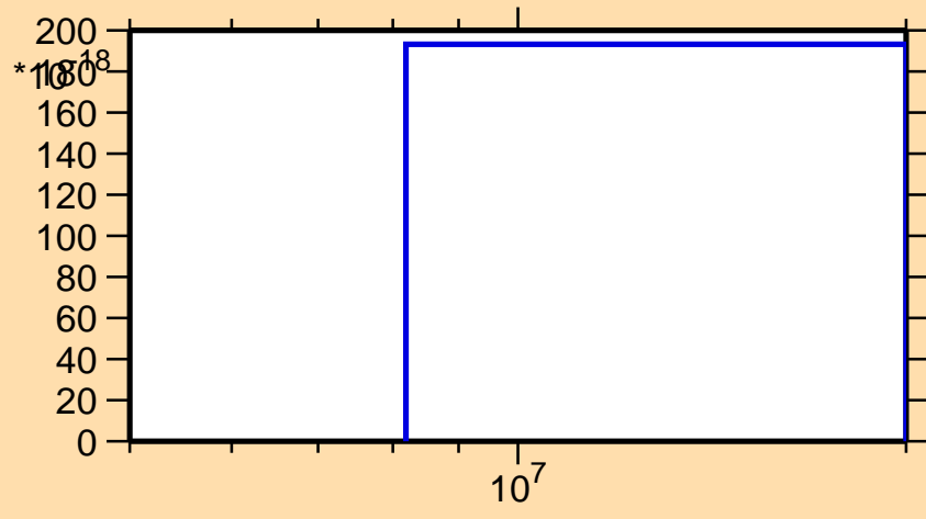
\sigma vs. E for ^{70}\text{Ge}(n,2np)
