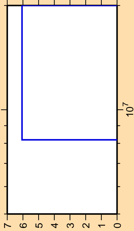
\Delta\sigma/\sigma vs. E for ^{70}\text{Ge}(n,2n)
