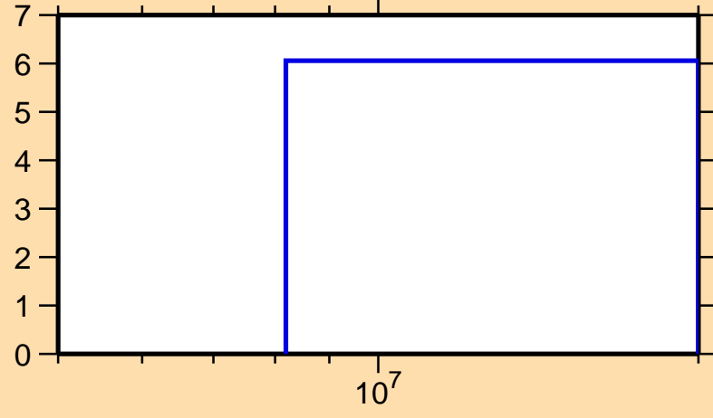
\Delta\sigma/\sigma vs. E for ^{70}\text{Ge}(n,2n)
