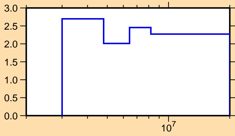
\Delta\sigma/\sigma vs. E for ^{70}\text{Ge}(n,n\text{inel.})
