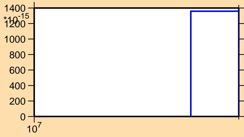
\sigma vs. E for ^{71}\text{Ge}(n,nt)
