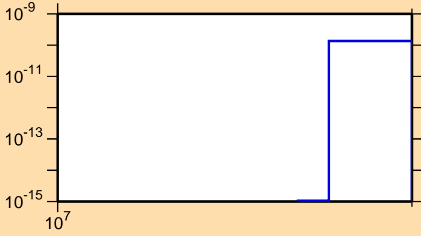
\sigma vs. E for ^{71}\text{Ge}(n,\text{pd})
