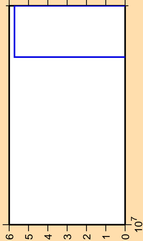
\Delta\sigma/\sigma vs. E for ^{71}\text{Ge}(n,nt)
