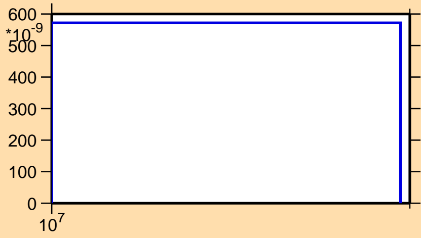
\sigma vs. E for ^{71}\text{Ge}(n,2n\alpha)
