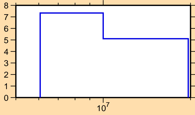
\Delta\sigma/\sigma vs. E for ^{71}\text{Ge}(n,2n)
