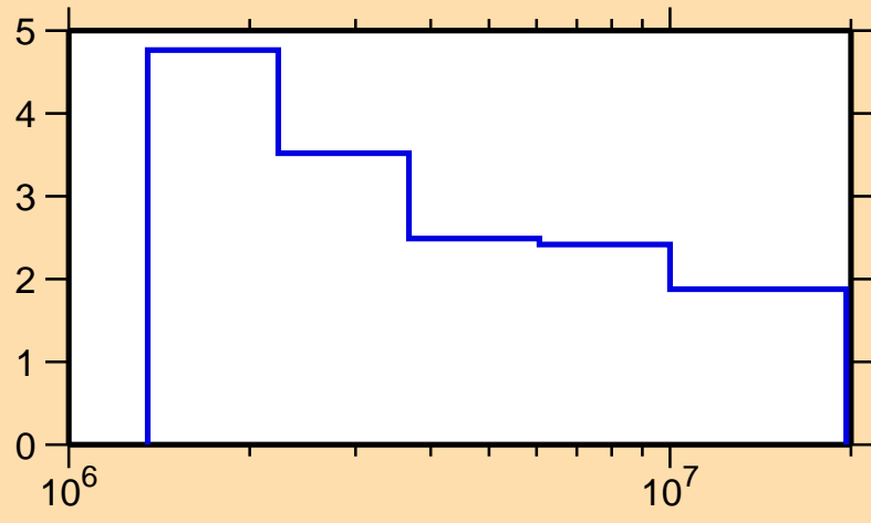
\Delta\sigma/\sigma vs. E for ^{71}\text{Ge}(n,n\text{onel.})
