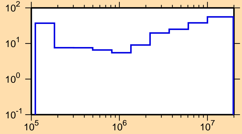
\Delta\sigma/\sigma vs. E for ^{71}\text{Ge}(n,n_1)
