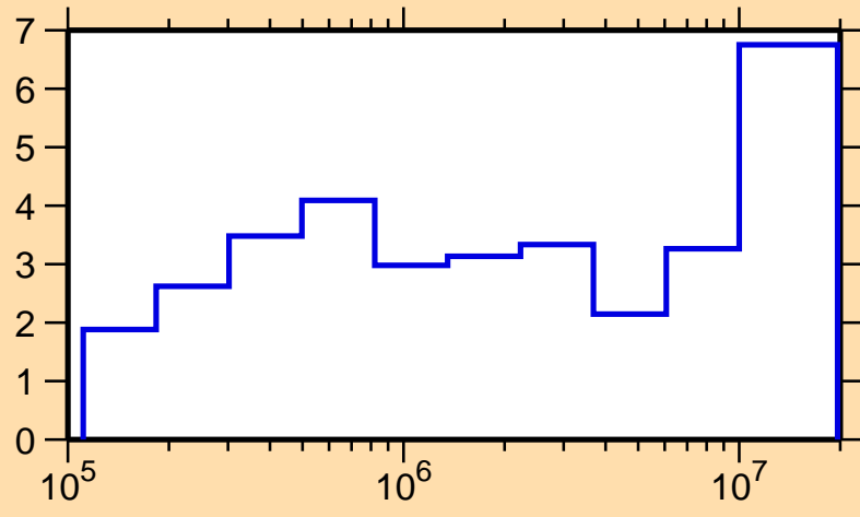
\Delta\sigma/\sigma vs. E for ^{71}\text{Ge}(n,\text{el.})
