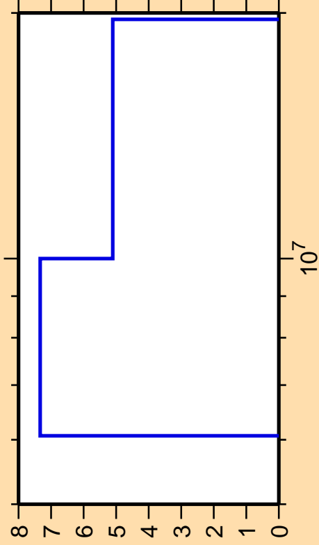
\Delta\sigma/\sigma vs. E for ^{71}\text{Ge}(n,2n)
