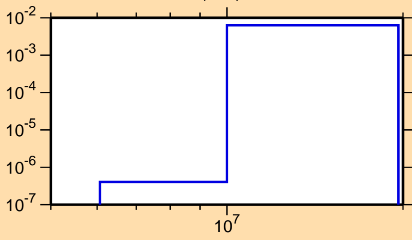
\sigma vs. E for ^{71}\text{Ge}(n,d)
