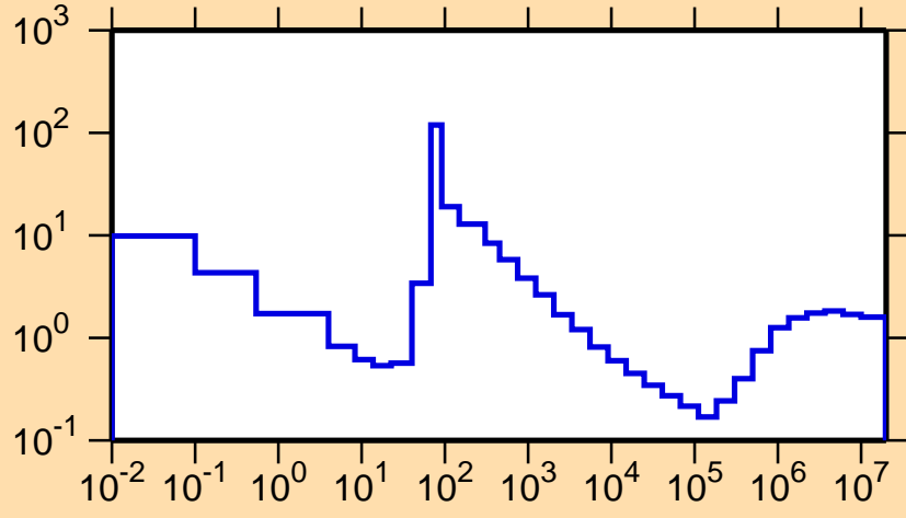
\sigma vs. E for ^{71}\text{Ge}(n,\text{nonel.})
