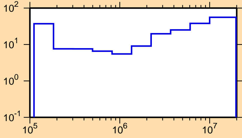
\Delta\sigma/\sigma vs. E for ^{71}\text{Ge}(n,n_1)
