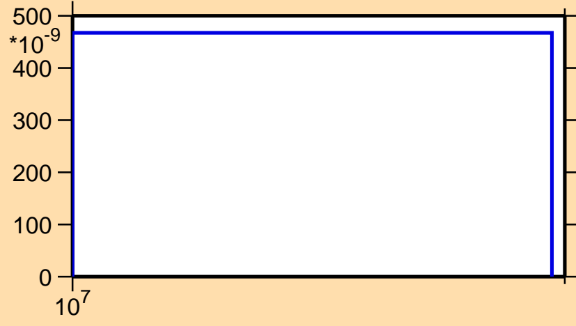
\sigma vs. E for ^{71}\text{Ge}(n,2np)
