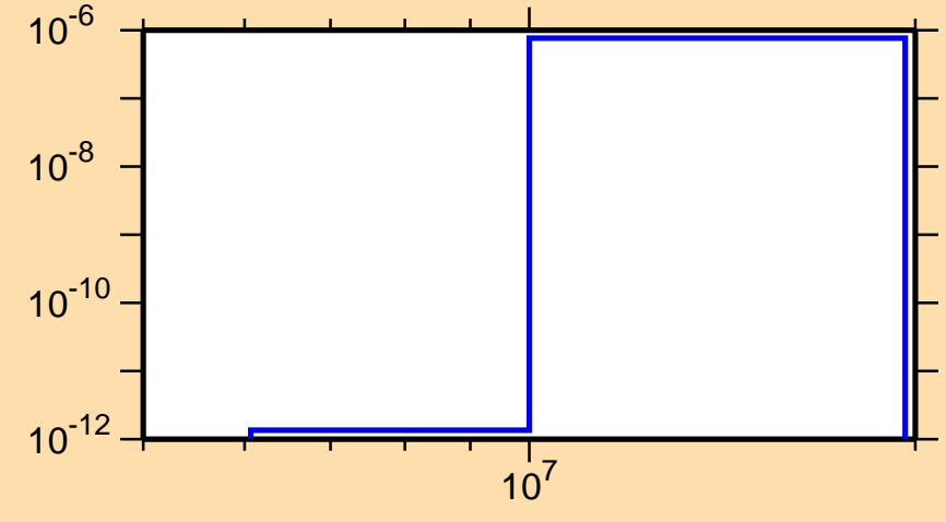
\sigma vs. E for ^{71}\text{Ge}(n,p\alpha)
