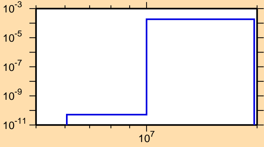
\sigma vs. E for ^{71}\text{Ge}(n,t)
