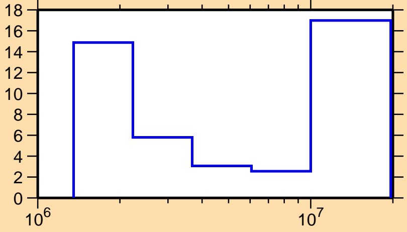
\Delta\sigma/\sigma vs. E for ^{71}\text{Ge}(n,n\text{cont.})
