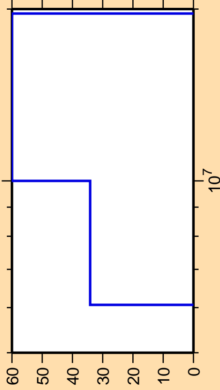
\Delta\sigma/\sigma vs. E for ^{71}\text{Ge}(n,t)
