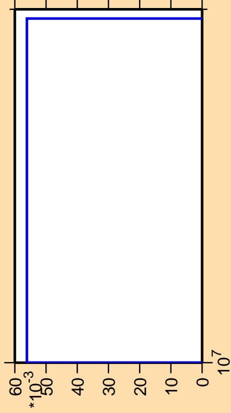
\Delta\sigma/\sigma vs. E for ^{71}\text{Ge}(n,nt)
