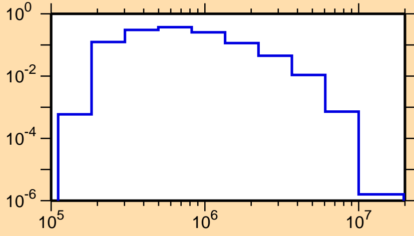
\sigma vs. E for ^{71}\text{Ge}(n,n_1)
