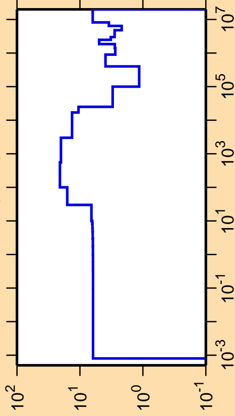
\Delta\sigma/\sigma vs. E for ^{71}\text{Ge}(n,\text{el.})
