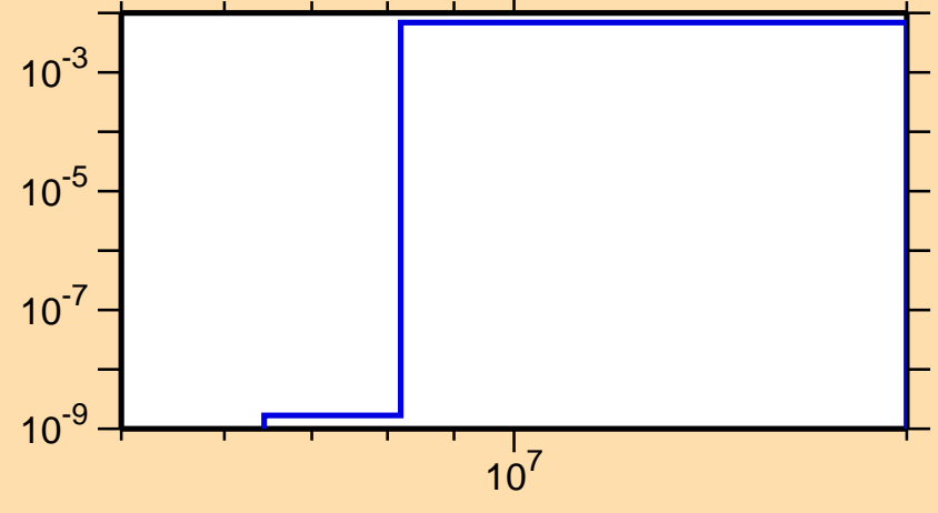
\sigma vs. E for ^{71}\text{Ge}(n,n\alpha)
