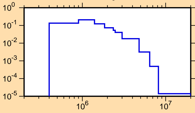
\sigma vs. E for ^{71}\text{Ge}(n,n_3)
