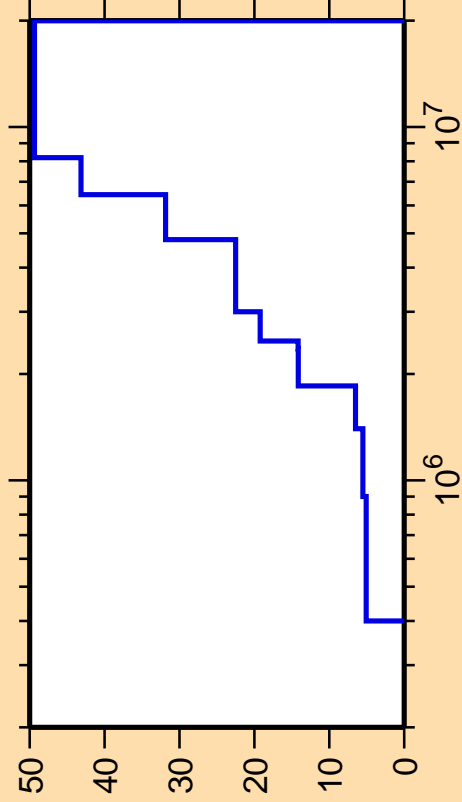
\Delta\sigma/\sigma vs. E for ^{71}\text{Ge}(n,n_4)
