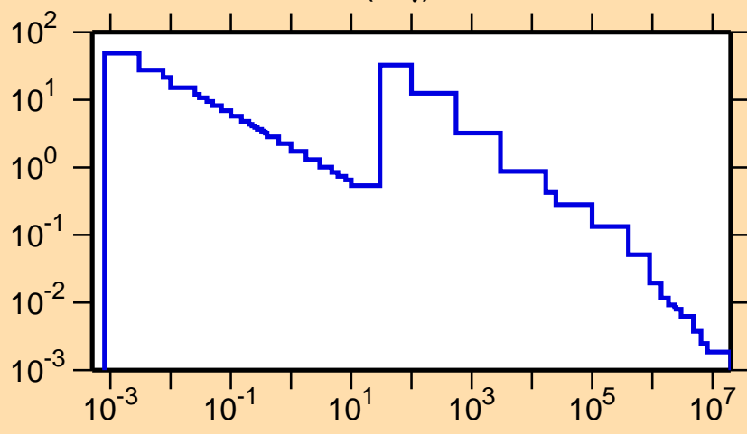
\sigma vs. E for ^{71}\text{Ge}(n,\gamma)
