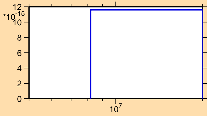
\sigma vs. E for ^{71}\text{Ge}(\text{mt117})
