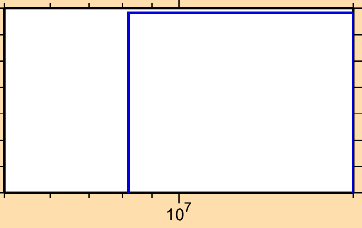
\sigma vs. E for ^{71}\text{Ge}(n,\text{nd})
