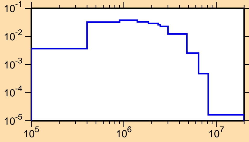
\sigma vs. E for ^{71}\text{Ge}(n,n_2)
