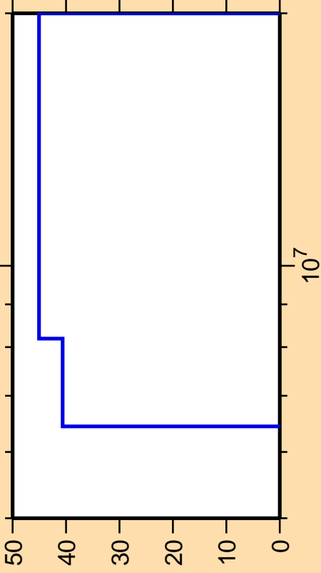
\Delta\sigma/\sigma vs. E for ^{71}\text{Ge}(n,\gamma)
