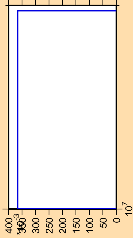
\Delta\sigma/\sigma vs. E for ^{72}\text{Ge}(n,2n\alpha)
