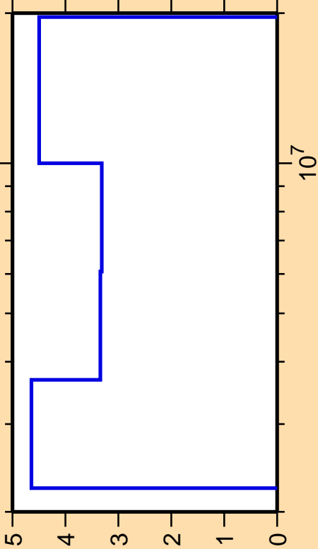
\Delta\sigma/\sigma vs. E for ^{72}\text{Ge}(n,n\text{cont.})
