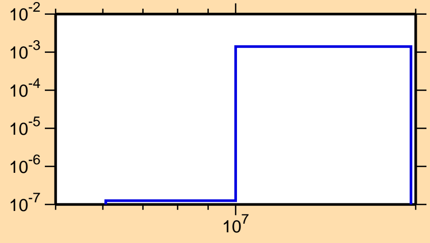
\sigma vs. E for ^{72}\text{Ge}(n,n\alpha)
