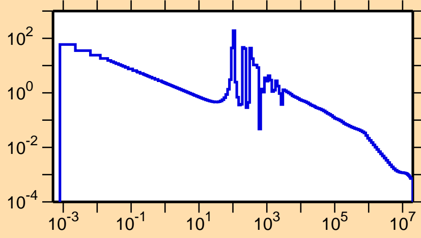
\sigma vs. E for ^{73}\text{Ge}(n,\gamma)
