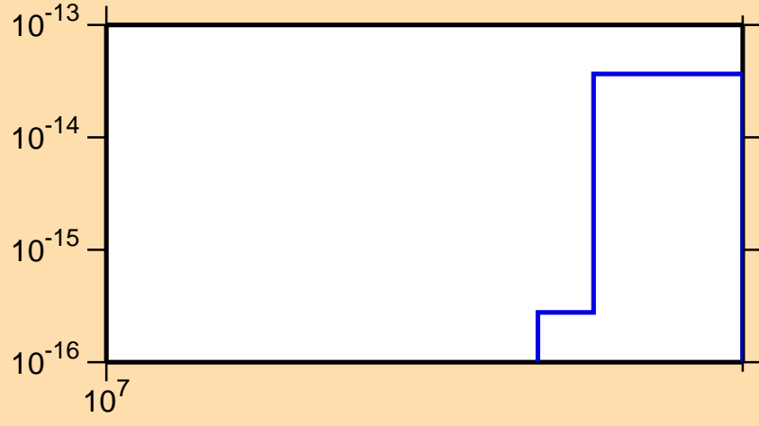
\sigma vs. E for ^{73}\text{Ge}(n,\text{pt})
