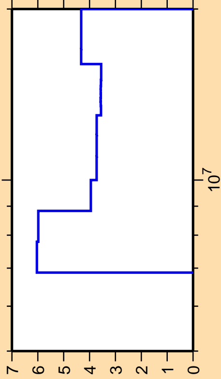
\Delta\sigma/\sigma vs. E for ^{73}\text{Ge}(n,2n)
