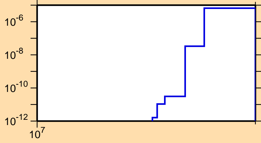
\sigma vs. E for ^{73}\text{Ge}(n,\text{nd})
