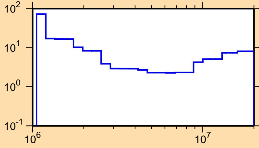
\Delta\sigma/\sigma vs. E for ^{73}\text{Ge}(n,n\text{cont.})
