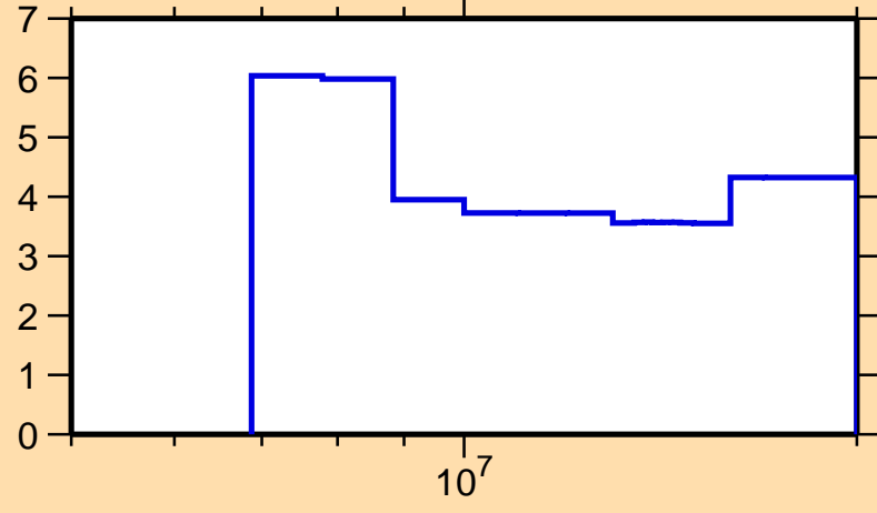
\Delta\sigma/\sigma vs. E for ^{73}\text{Ge}(n,2n)
