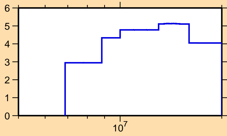
\Delta\sigma/\sigma vs. E for ^{73}\text{Ge}(n,\text{el.})
