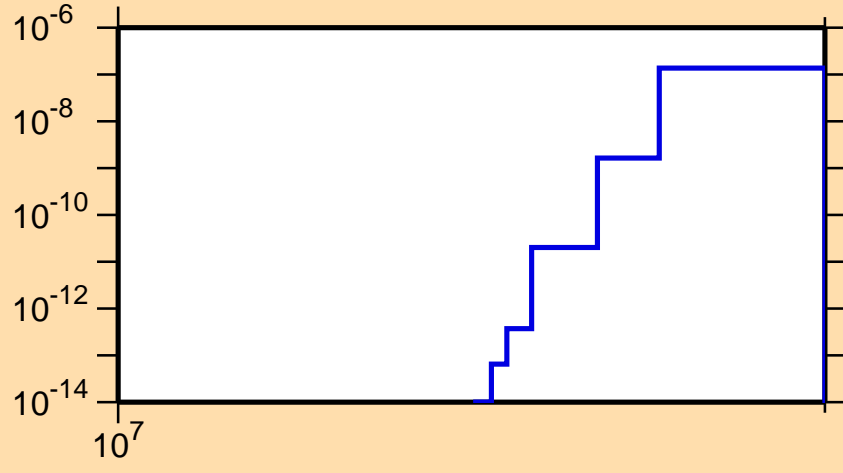
\sigma vs. E for ^{73}\text{Ge}(n,\text{He3})
