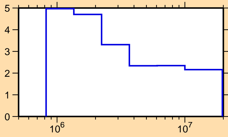
\Delta\sigma/\sigma vs. E for ^{73}\text{Ge}(n,n\text{onel.})
