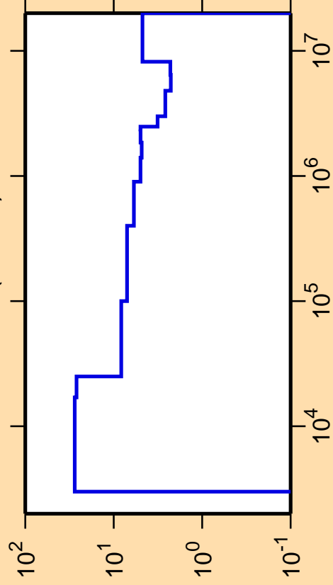
\Delta\sigma/\sigma vs. E for ^{73}\text{Ge}(n,\text{inel.})
