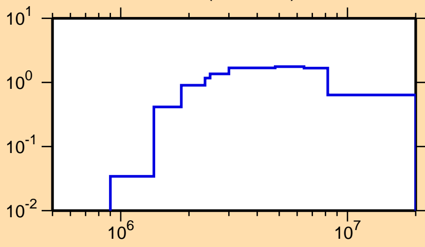
\sigma vs. E for ^{73}\text{Ge}(n,n\text{cont.})
