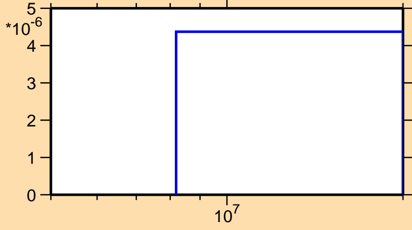
\sigma vs. E for ^{73}\text{Ge}(n,3n)
