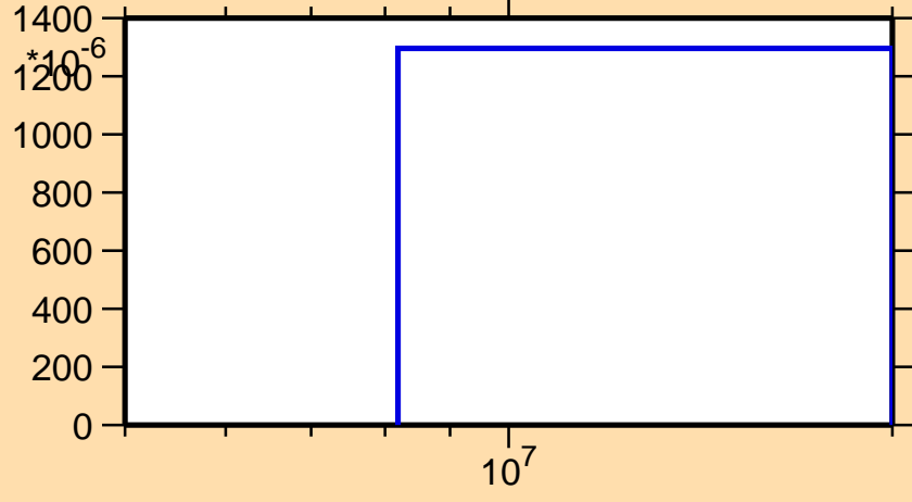
\sigma vs. E for ^{73}\text{Ge}(n,d)
