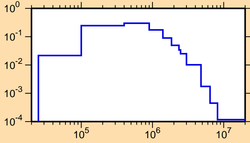
\sigma vs. E for ^{73}\text{Ge}(n,n_3)
