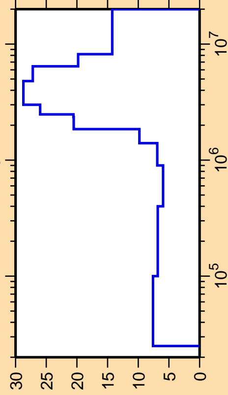
\Delta\sigma/\sigma vs. E for ^{73}\text{Ge}(n,n_3)
