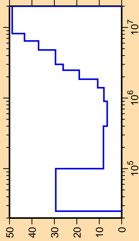
\Delta\sigma/\sigma vs. E for ^{73}\text{Ge}(n,n_2)
