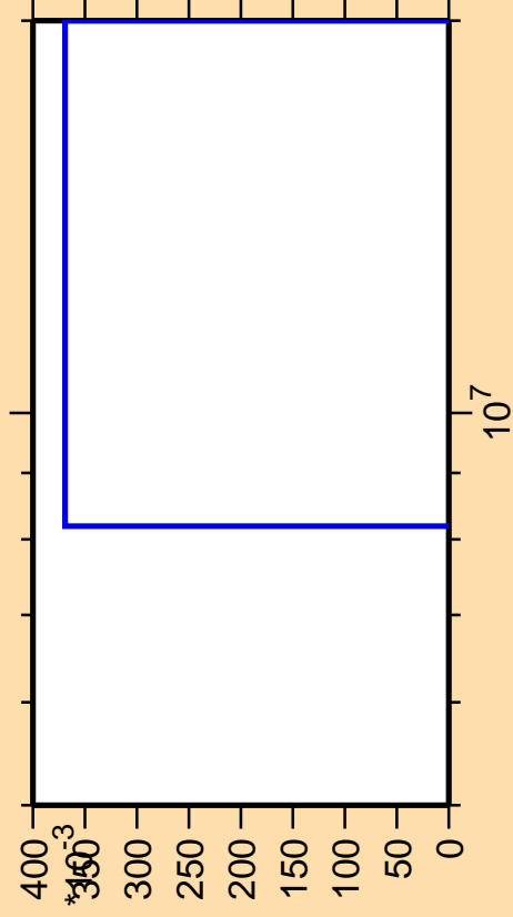
\Delta\sigma/\sigma vs. E for ^{73}\text{Ge}(n,nt)
