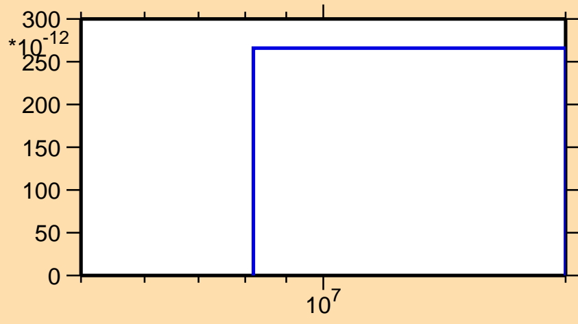
\sigma vs. E for ^{73}\text{Ge}(n,p\alpha)
