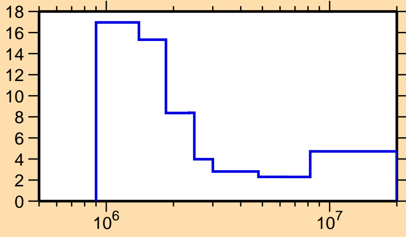
\Delta\sigma/\sigma vs. E for ^{73}\text{Ge}(n,ncont.)
