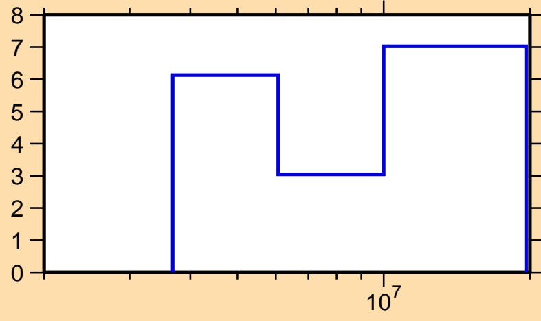
\Delta\sigma/\sigma vs. E for ^{74}\text{Ge}(n,n\text{cont.})
