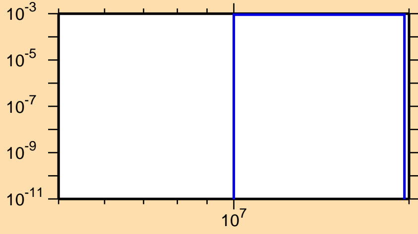
\sigma vs. E for ^{74}\text{Ge}(n,d)
