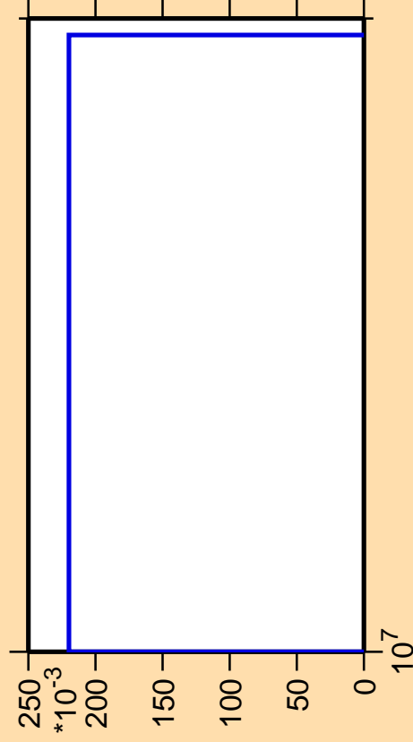
\Delta\sigma/\sigma vs. E for ^{74}\text{Ge}(n,\text{nd})
