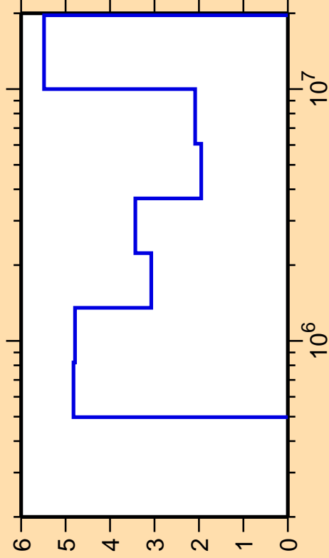
\Delta\sigma/\sigma vs. E for ^{74}\text{Ge}(n,\text{inel.})
