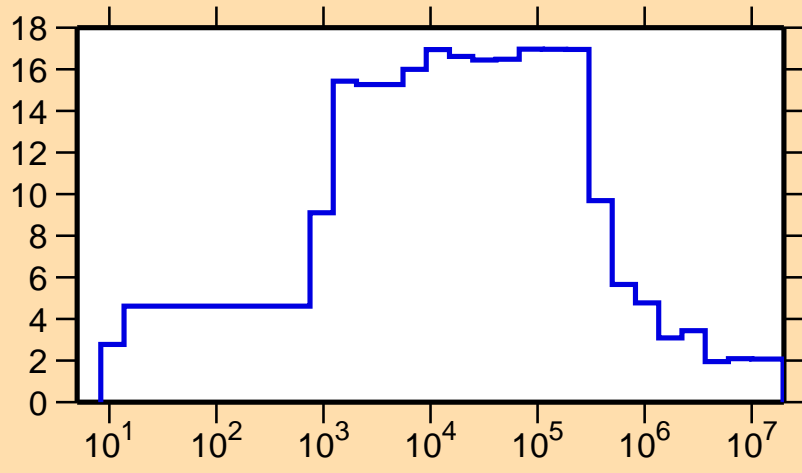
\Delta\sigma/\sigma vs. E for ^{74}\text{Ge}(n,\text{nonel.})
