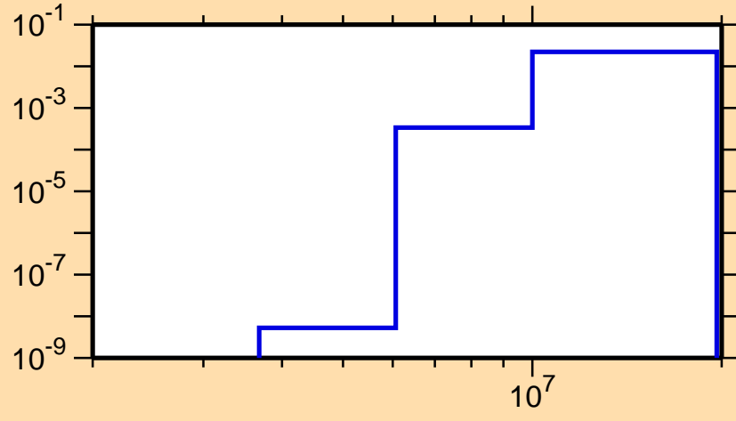
\sigma vs. E for ^{74}\text{Ge}(n,p)
