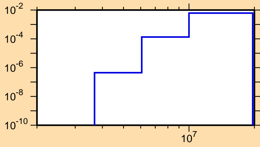
\sigma vs. E for ^{74}\text{Ge}(n,\alpha)
