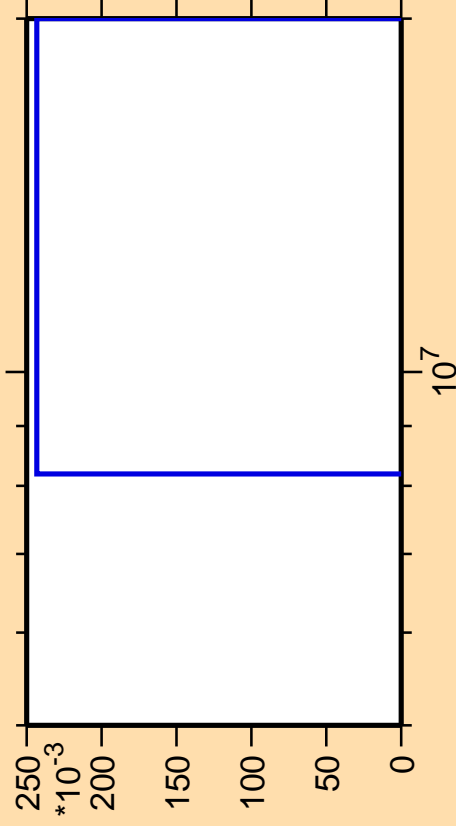
\Delta\sigma/\sigma vs. E for ^{74}\text{Ge}(n,nd)
