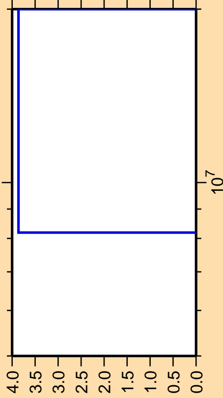
\Delta\sigma/\sigma vs. E for ^{74}\text{Ge}(n,2n)
