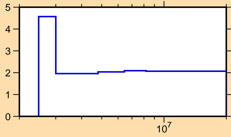
\Delta\sigma/\sigma vs. E for ^{74}\text{Ge}(n,n\text{onel.})
