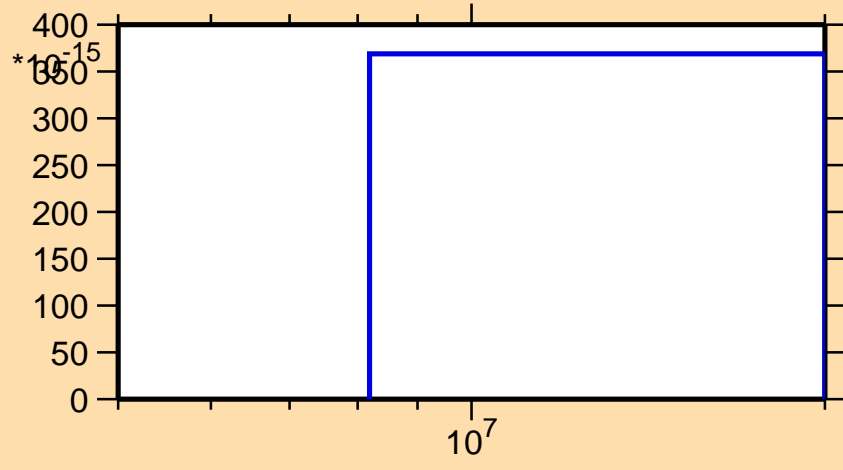
\sigma vs. E for ^{74}\text{Ge}(n,nd)
