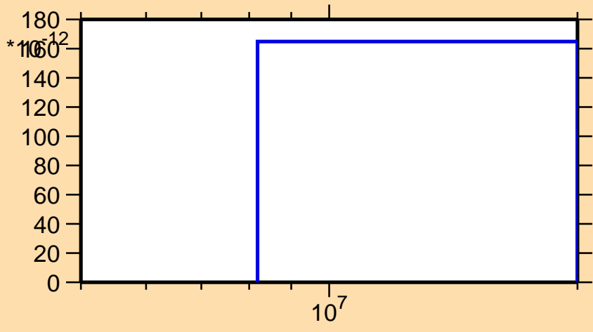
\sigma vs. E for ^{75}\text{Ge}(n,2n\alpha)
