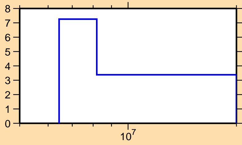
\Delta\sigma/\sigma vs. E for ^{75}\text{Ge}(n,2n)
