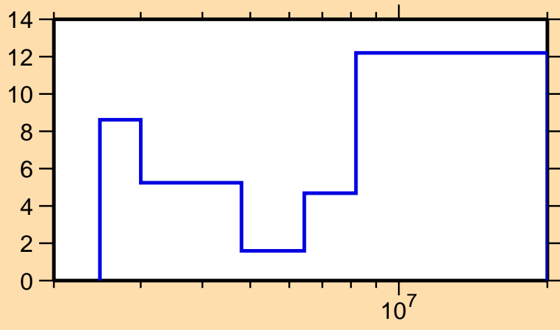
\Delta\sigma/\sigma vs. E for ^{75}\text{Ge}(n,n\text{cont.})
