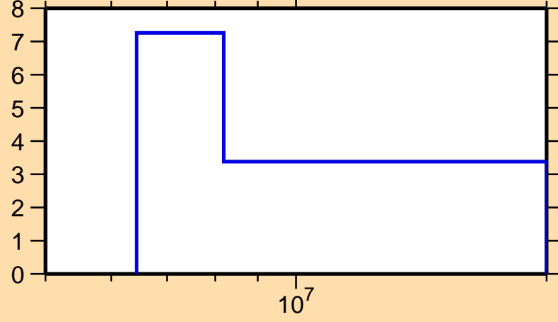
\Delta\sigma/\sigma vs. E for ^{75}\text{Ge}(n,2n)
