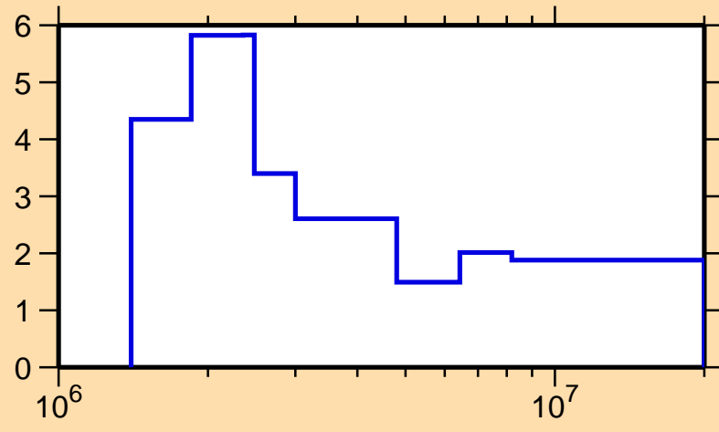
\Delta\sigma/\sigma vs. E for ^{75}\text{Ge}(n,n\text{onel.})
