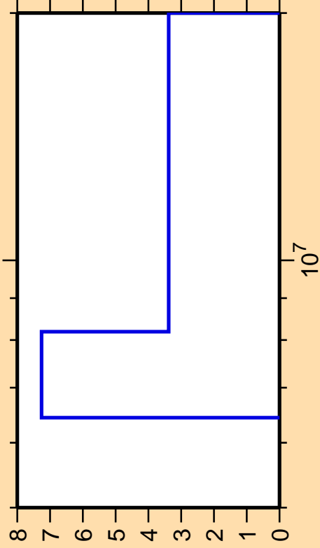
\Delta\sigma/\sigma vs. E for ^{75}\text{Ge}(n,2n)
