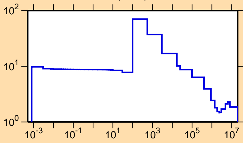
\sigma vs. E for ^{75}\text{Ge}(n,\text{el.})
