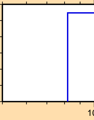
\sigma vs. E for ^{75}\text{Ge}(n,\text{pd})
