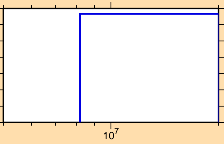
\sigma vs. E for ^{75}\text{Ge}(n,n\alpha)
