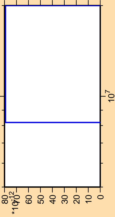
\Delta\sigma/\sigma vs. E for ^{75}\text{Ge} (mt 34)
