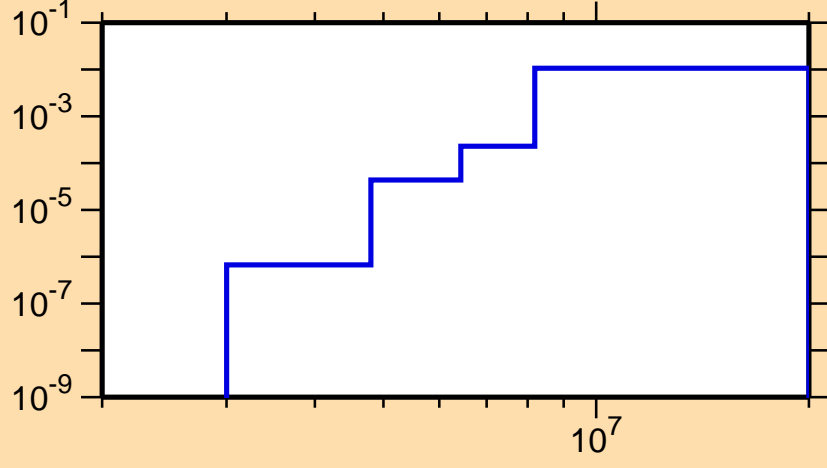
\sigma vs. E for ^{75}\text{Ge}(n,p)
