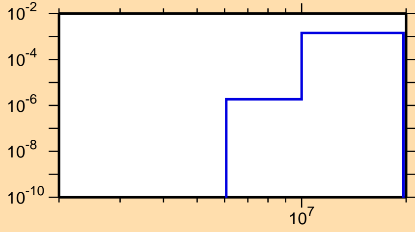
\sigma vs. E for ^{76}\text{Ge}(n,\alpha)
