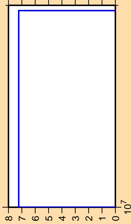
\Delta\sigma/\sigma vs. E for ^{76}\text{Ge}(n,3n)
