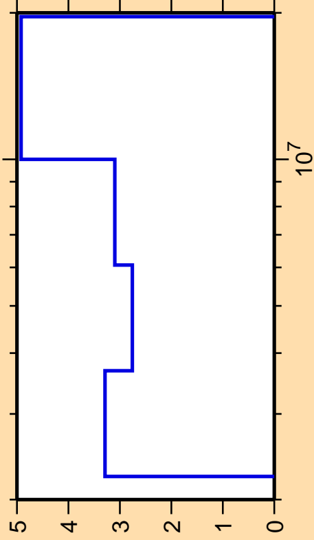
\Delta\sigma/\sigma vs. E for ^{76}\text{Ge}(n,n\text{cont.})
