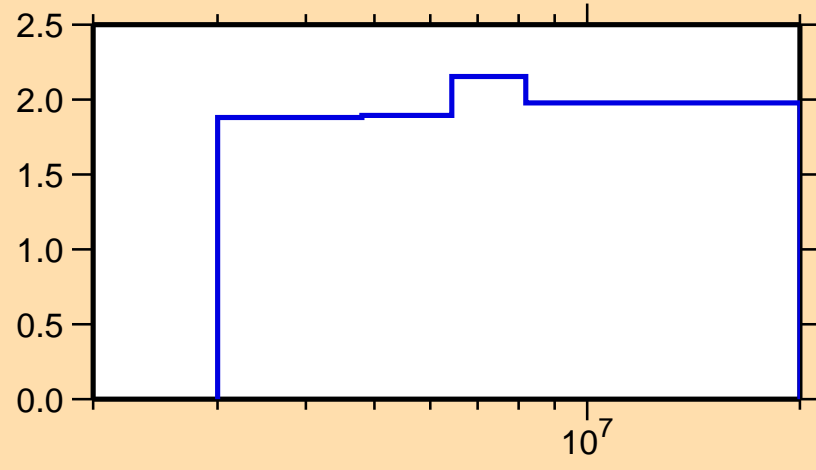
\Delta\sigma/\sigma vs. E for ^{76}\text{Ge}(n,n\text{nonel.})
