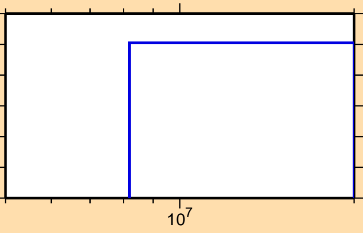
\sigma vs. E for ^{76}\text{Ge}(n,3n)
