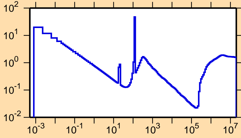
\sigma vs. E for ^{77}\text{Ge}(n,\text{nonel.})
