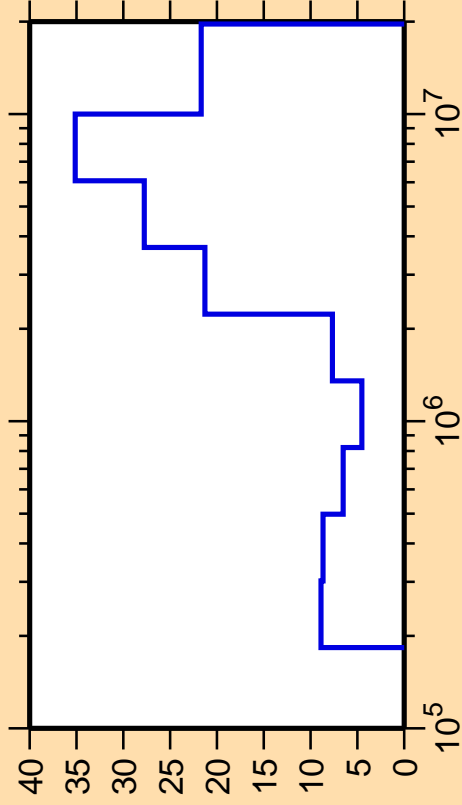
\Delta\sigma/\sigma vs. E for ^{77}\text{Ge}(n,n_2)
