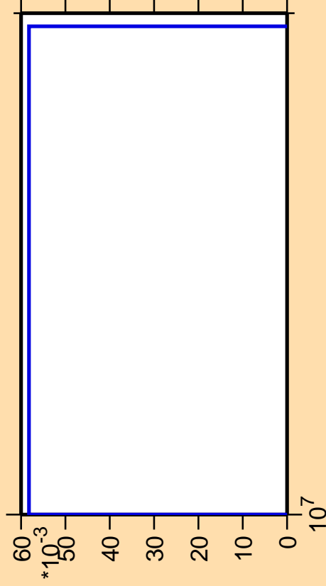
\Delta\sigma/\sigma vs. E for ^{77}\text{Ge}(n,2np)
