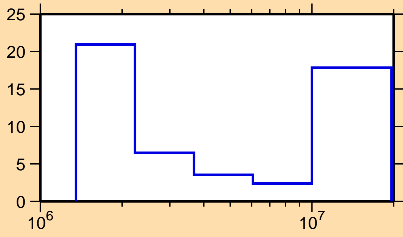
\Delta\sigma/\sigma vs. E for ^{77}\text{Ge}(n,n\text{cont.})
