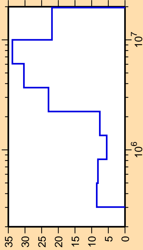
\Delta\sigma/\sigma vs. E for ^{77}\text{Ge}(n,n_3)
