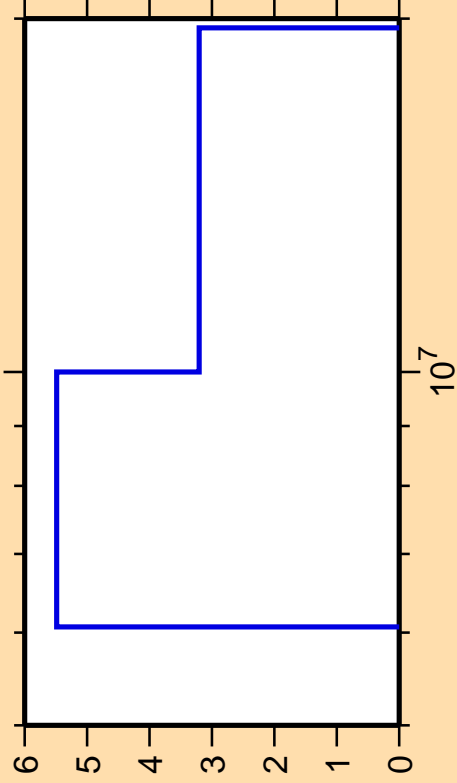
\Delta\sigma/\sigma vs. E for ^{77}\text{Ge}(n,2n)
