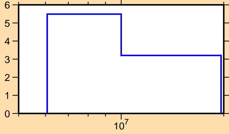
\Delta\sigma/\sigma vs. E for ^{77}\text{Ge}(n,2n)
