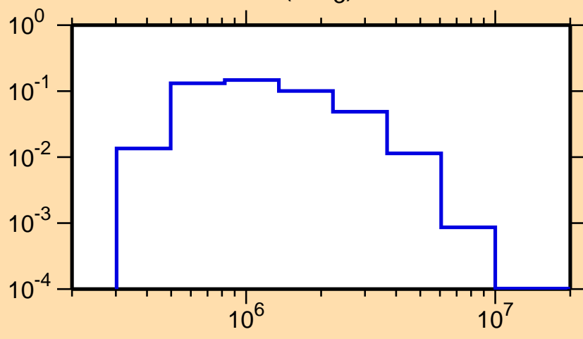
\sigma vs. E for ^{77}\text{Ge}(n,n_3)
