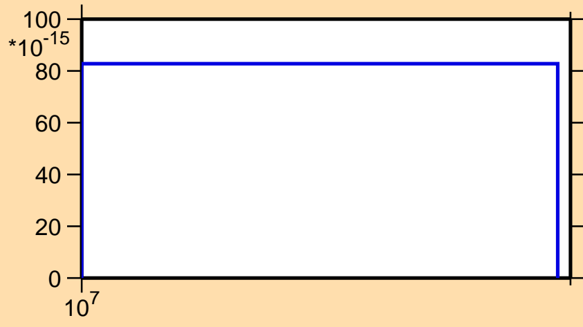
\sigma vs. E for ^{77}\text{Ge}(n,2np)
