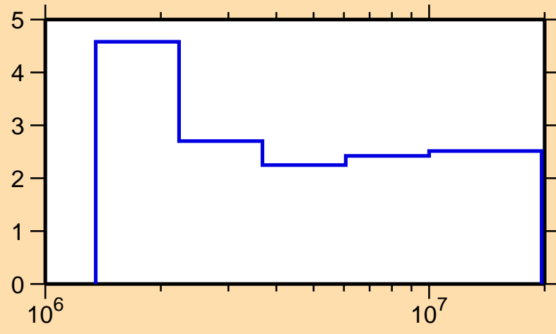
\Delta\sigma/\sigma vs. E for ^{77}\text{Ge}(n,\text{nonel.})
