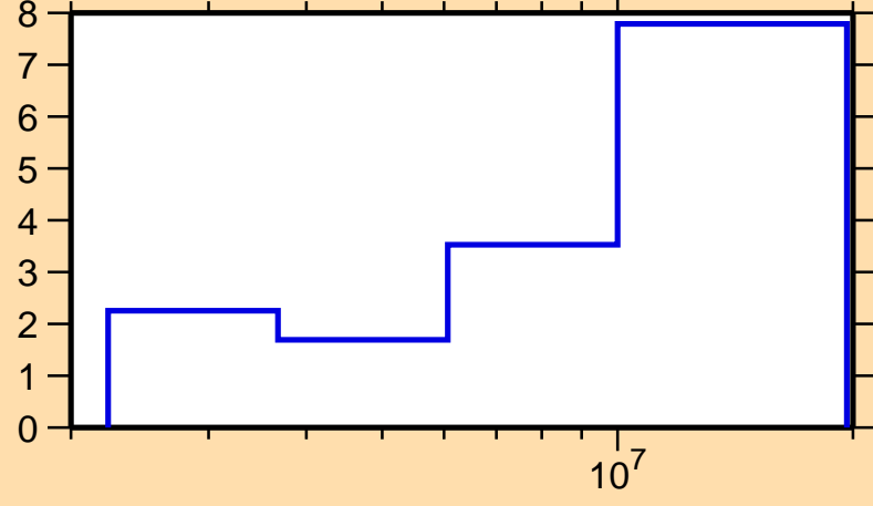
\Delta\sigma/\sigma vs. E for ^{77}\text{Ge}(n,\text{el.})
