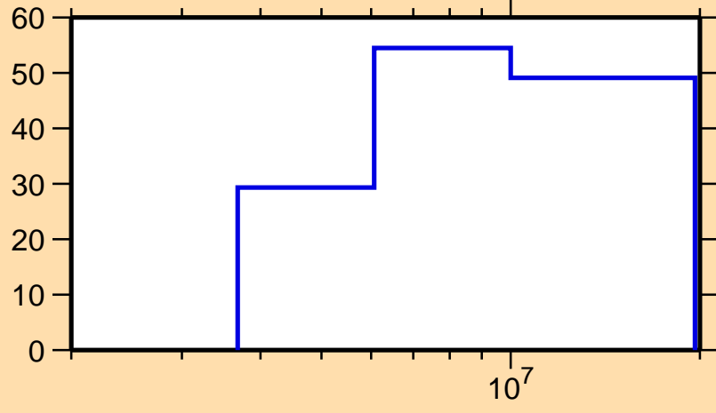
\Delta\sigma/\sigma vs. E for ^{77}\text{Ge}(n,p)
