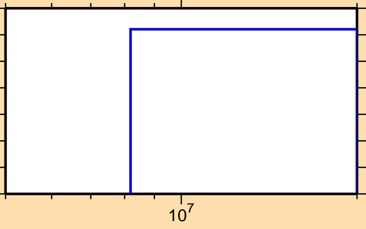
\sigma vs. E for ^{77}\text{Ge}(n,2np)
