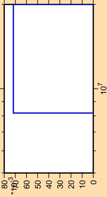
\Delta\sigma/\sigma vs. E for ^{77}\text{Ge}(n,2np)
