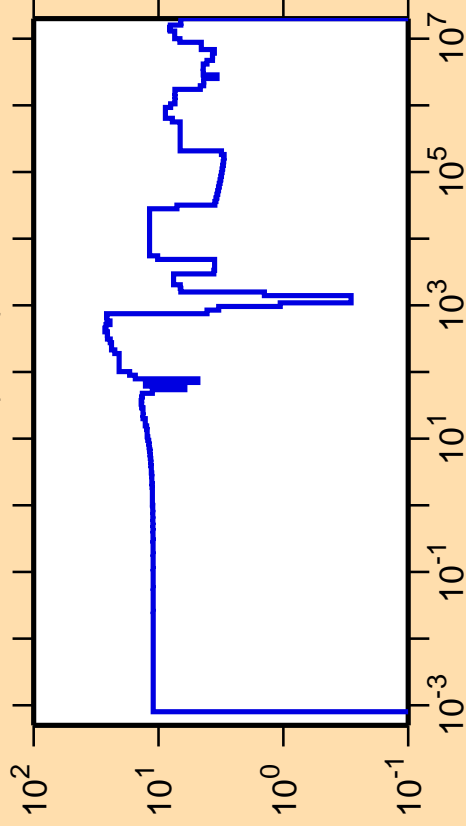
\Delta\sigma/\sigma vs. E for ^{77}\text{Ge}(n,\text{el.})
