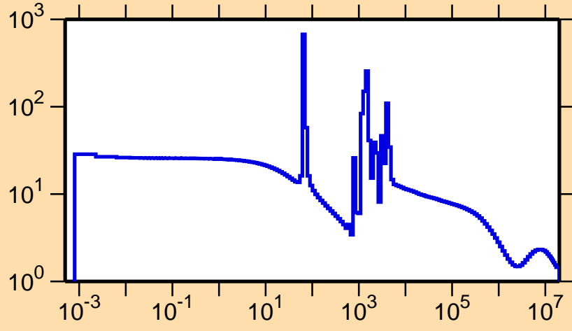
\sigma vs. E for ^{77}\text{Ge}(n,\text{el.})
