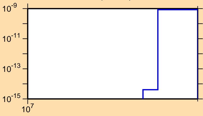
\sigma vs. E for ^{77}\text{Ge}(n,2n\alpha)
