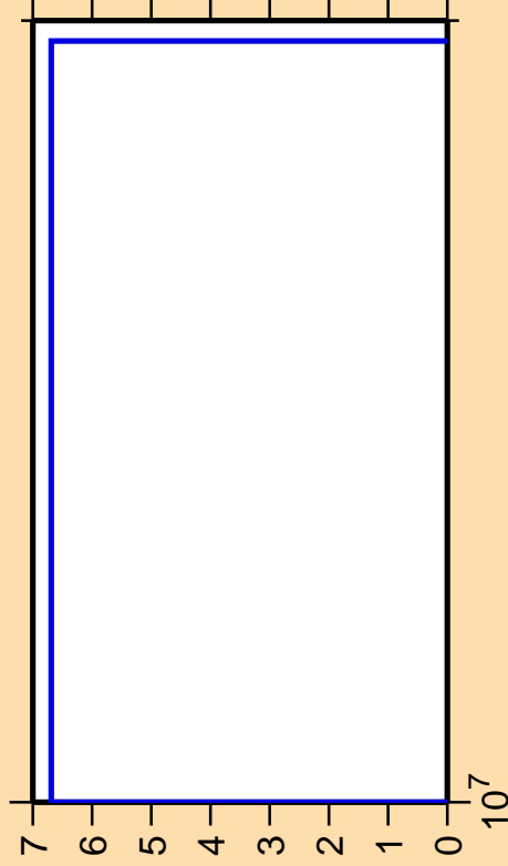
\Delta\sigma/\sigma vs. E for ^{77}\text{Ge}(n,3n)
