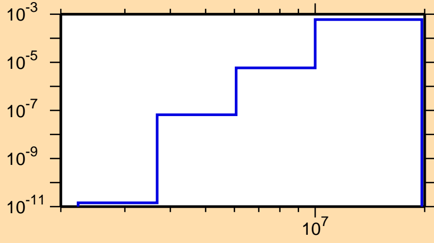
\sigma vs. E for ^{77}\text{Ge}(n,\alpha)
