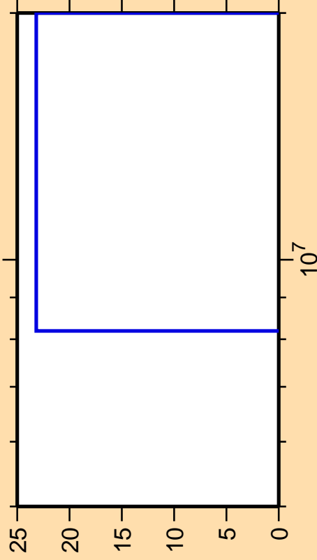
\Delta\sigma/\sigma vs. E for ^{77}\text{Ge}(n,np)
