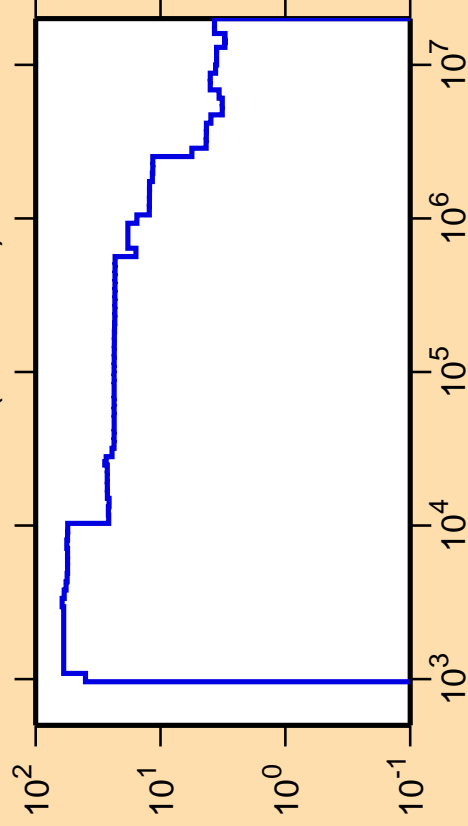
\Delta\sigma/\sigma vs. E for ^{78}\text{Ge}(n,\text{nonel.})
