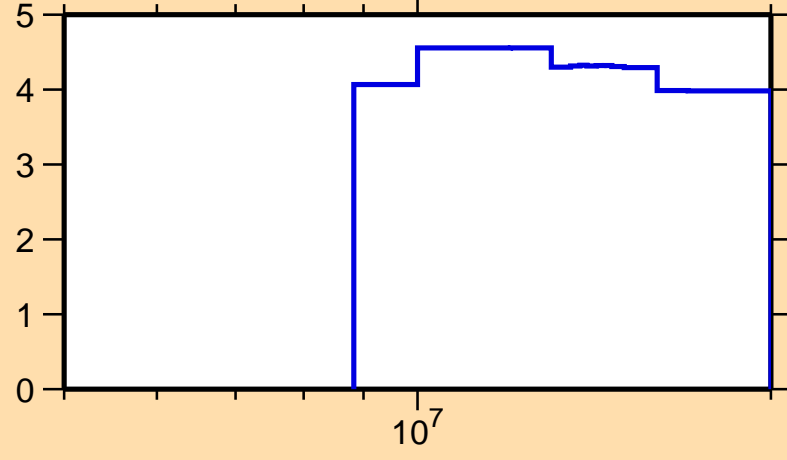
\Delta\sigma/\sigma vs. E for ^{78}\text{Ge}(n,\text{tot.})
