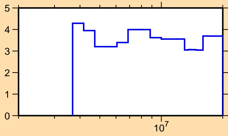
\Delta\sigma/\sigma vs. E for ^{78}\text{Ge}(n,n\text{inel.})
