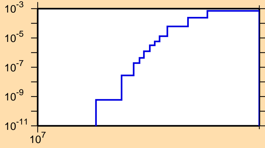
\sigma vs. E for ^{78}\text{Ge}(n,d)
