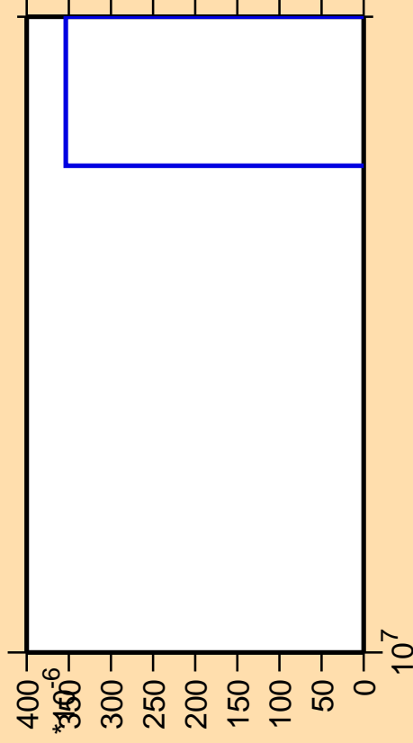
\Delta\sigma/\sigma vs. E for ^{78}\text{Ge}(n,nd)
