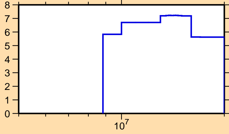
\Delta\sigma/\sigma vs. E for ^{78}\text{Ge}(n,\text{el.})
