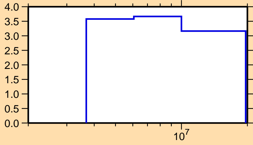
\Delta\sigma/\sigma vs. E for ^{78}\text{Ge}(n,n\text{onel.})
