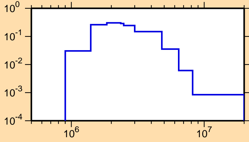
\sigma vs. E for ^{78}\text{Ge}(n,n_2)
