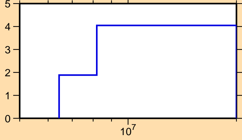
\Delta\sigma/\sigma vs. E for ^{78}\text{Ge}(n,\text{tot.})
