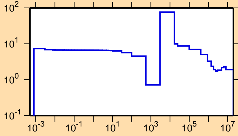
\sigma vs. E for ^{78}\text{Ge}(n,\text{el.})
