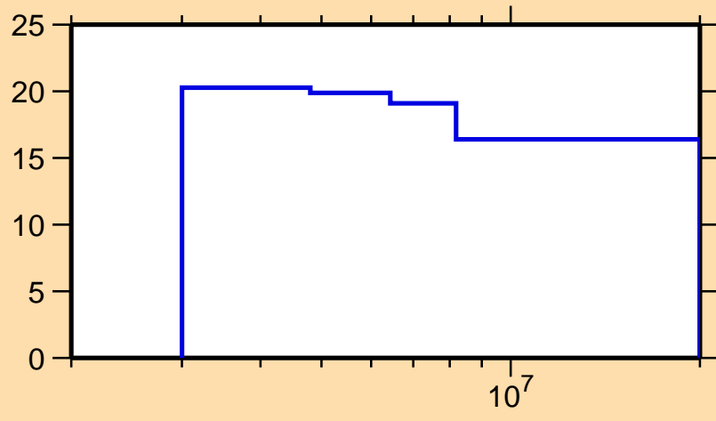
\Delta\sigma/\sigma vs. E for ^{78}\text{Ge}(n, n_1)
