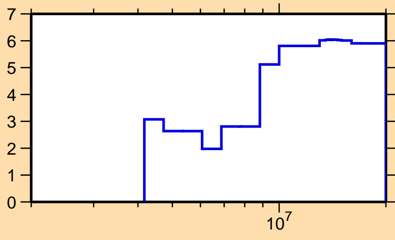
\Delta\sigma/\sigma vs. E for ^{79}\text{Ge}(n,\text{tot.})
