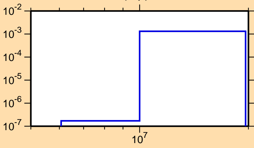
\sigma vs. E for ^{79}\text{Ge}(n,p)
