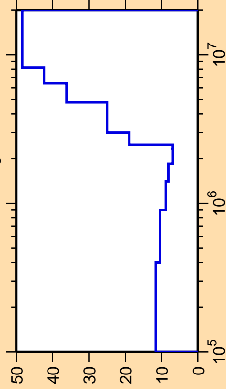
\Delta\sigma/\sigma vs. E for ^{79}\text{Ge}(n,n_3)
