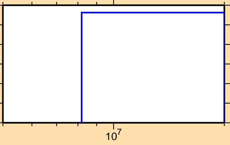
\sigma vs. E for ^{79}\text{Ge}(n,3n)
