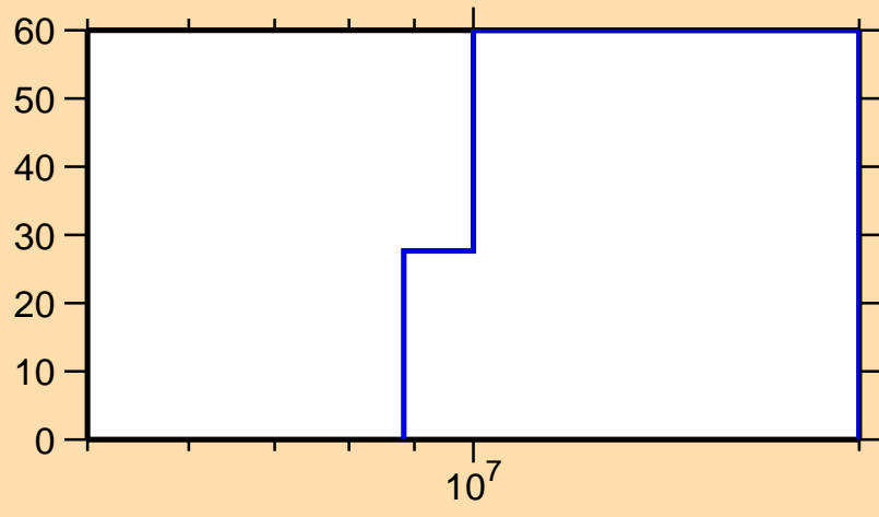
\Delta\sigma/\sigma vs. E for ^{80}\text{Ge}(n,p)
