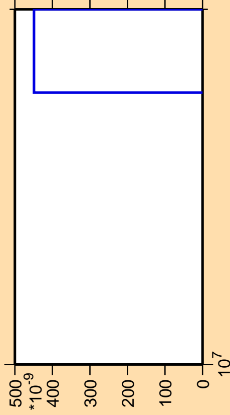
\Delta\sigma/\sigma vs. E for ^{80}\text{Ge}(n,\text{nd})
