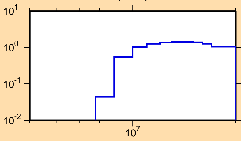
\sigma vs. E for ^{80}\text{Ge}(n,2n)
