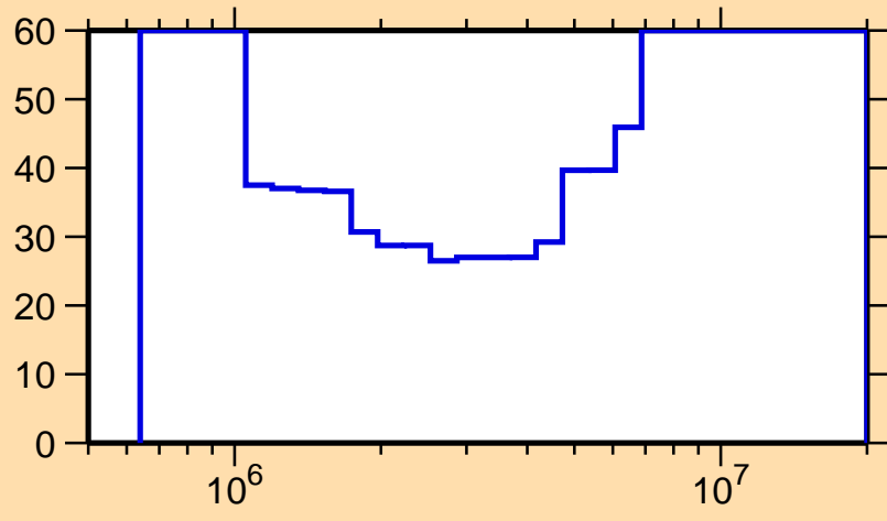
\Delta\sigma/\sigma vs. E for ^{80}\text{Ge}(n,n_1)
