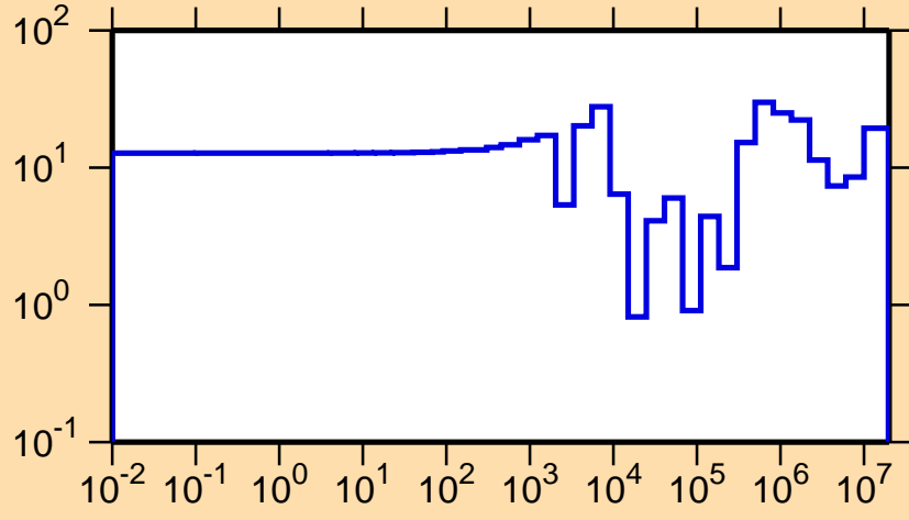
\Delta\sigma/\sigma vs. E for ^{80}\text{Ge}(n,\text{el.})
