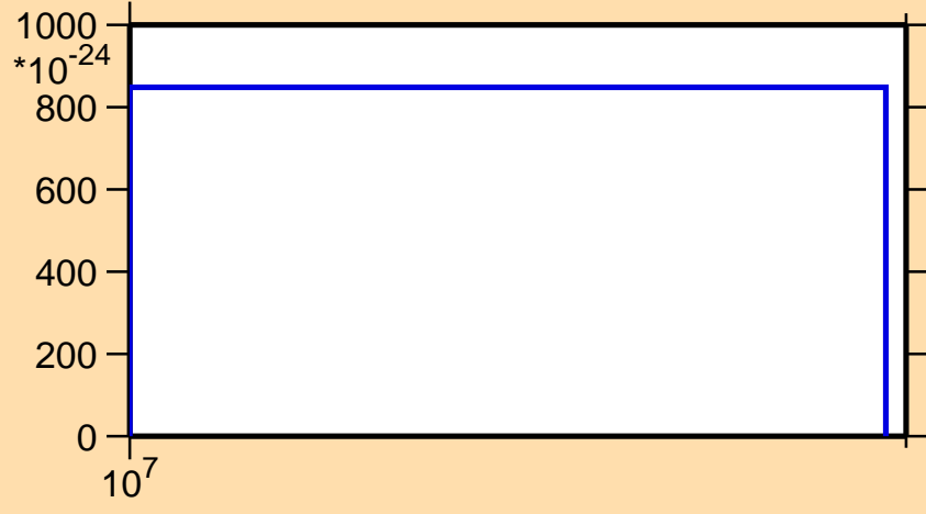
\sigma vs. E for ^{80}\text{Ge}(n,nd)
