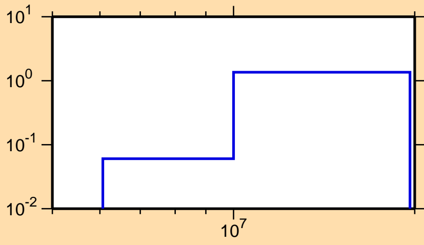
\sigma vs. E for ^{80}\text{Ge}(n,2n)
