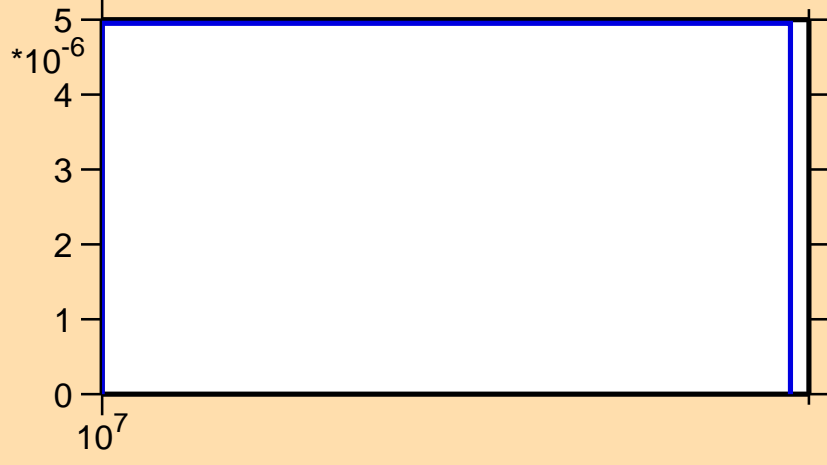
\sigma vs. E for ^{80}\text{Ge}(n,d)
