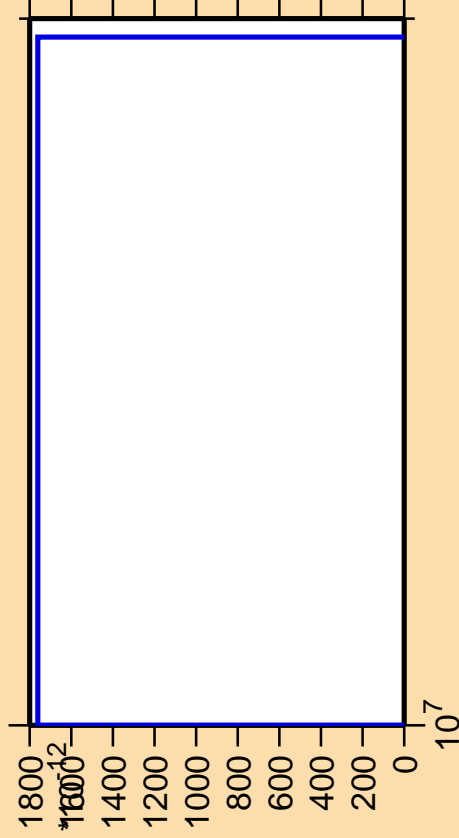
\Delta\sigma/\sigma vs. E for ^{80}\text{Ge}(n,nd)
