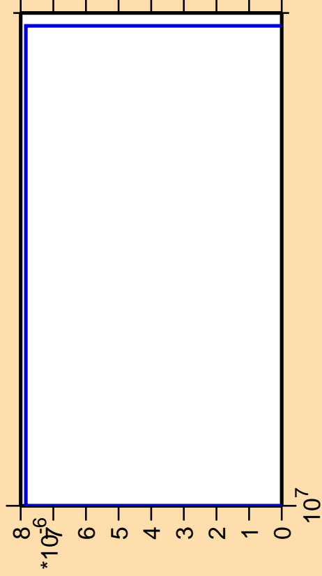
\Delta\sigma/\sigma vs. E for ^{80}\text{Ge}(n,nt)
