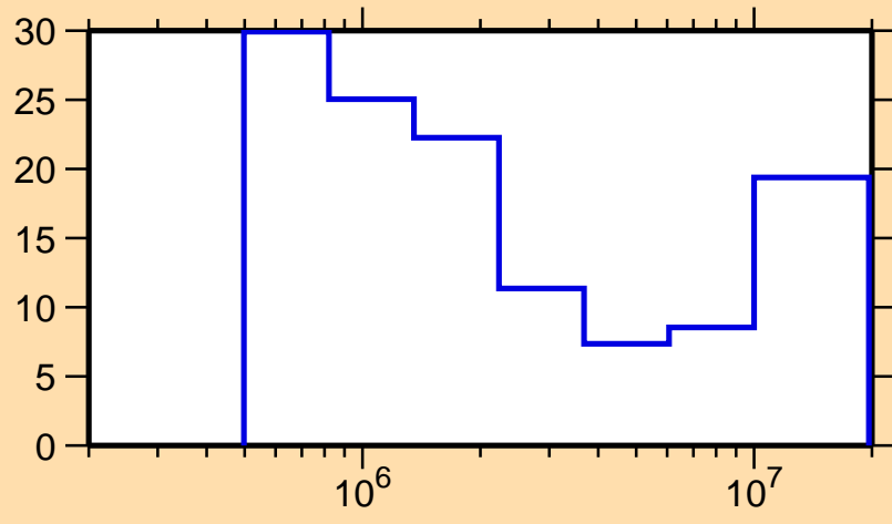
\Delta\sigma/\sigma vs. E for ^{80}\text{Ge}(n,\text{el.})
