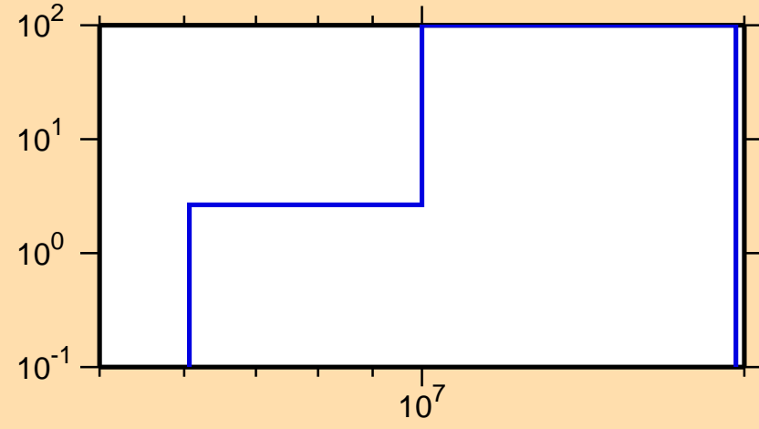
\Delta\sigma/\sigma vs. E for ^{80}\text{Ge}(n,p)
