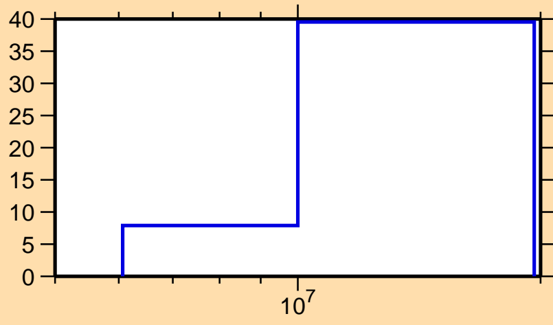
\Delta\sigma/\sigma vs. E for ^{80}\text{Ge}(n,\text{inel.})
