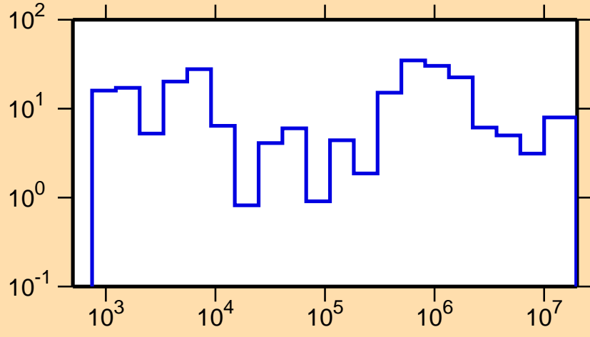
\Delta\sigma/\sigma vs. E for ^{80}\text{Ge}(n,\text{tot.})
