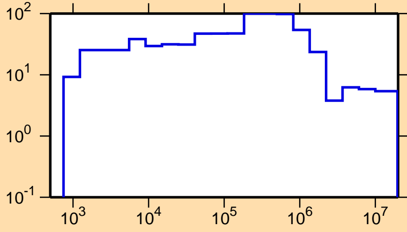
\Delta\sigma/\sigma vs. E for ^{80}\text{Ge}(n,\text{nonel.})
