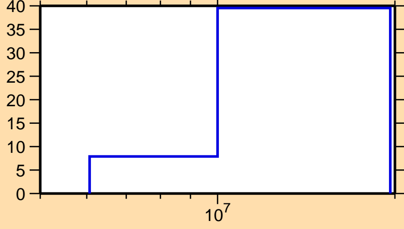
\Delta\sigma/\sigma vs. E for ^{80}\text{Ge}(n,\text{inel.})
