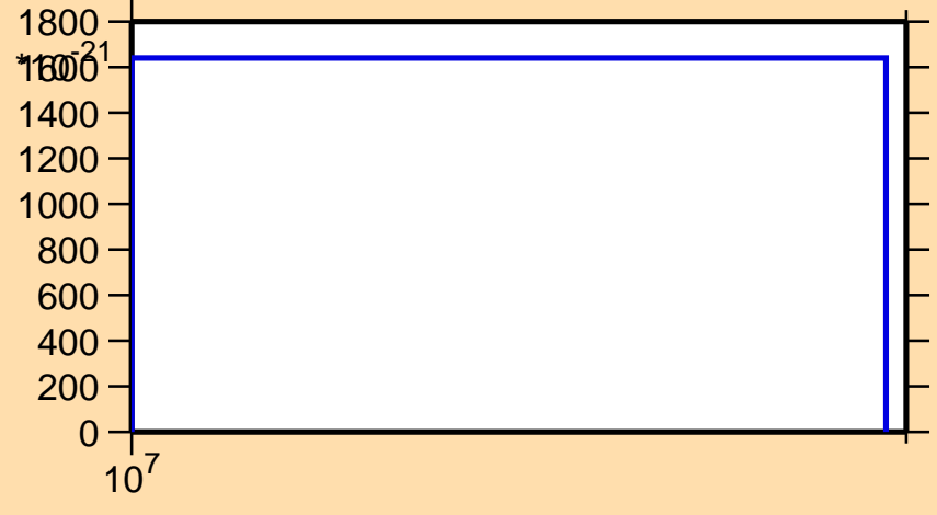
\sigma vs. E for ^{80}\text{Ge}(n,nt)
