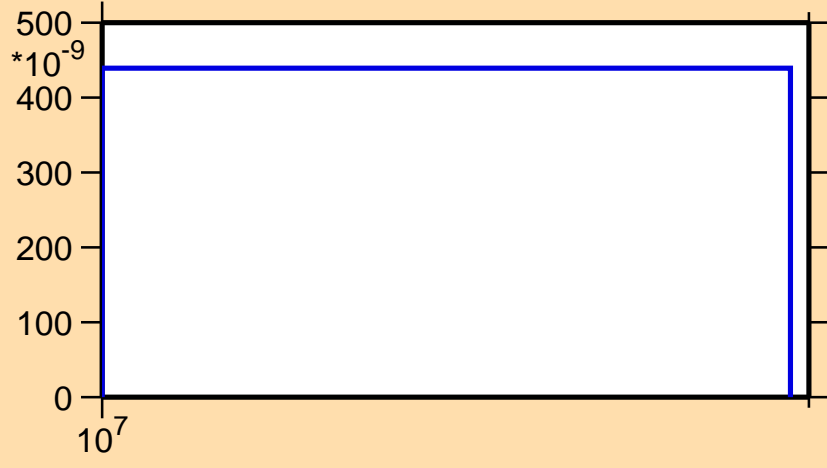
\sigma vs. E for ^{80}\text{Ge}(n,np)
