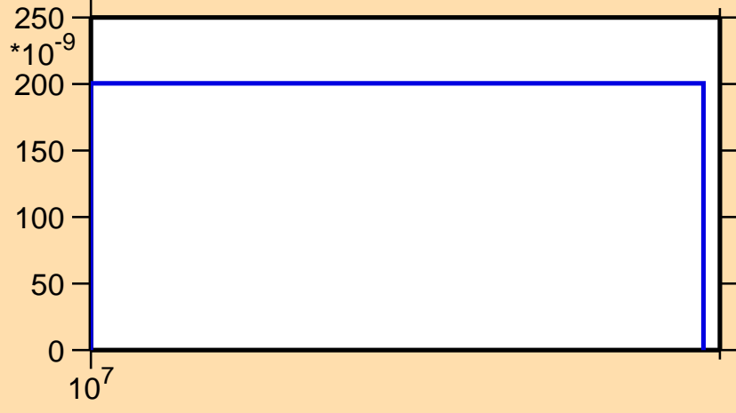
\sigma vs. E for ^{80}\text{Ge}(n,t)
