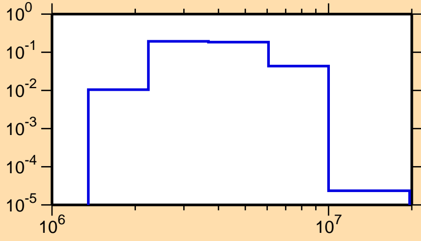
\sigma vs. E for ^{80}\text{Ge}(n,n_4)
