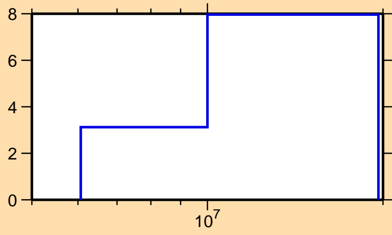
\Delta\sigma/\sigma vs. E for ^{80}\text{Ge}(n,\text{tot.})
