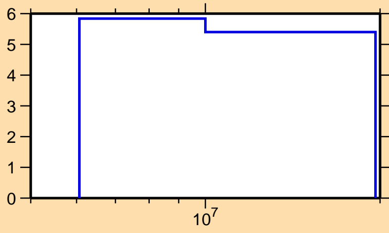
\Delta\sigma/\sigma vs. E for ^{80}\text{Ge}(n,\text{nonel.})
