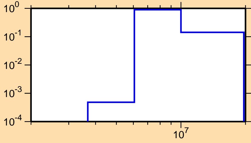
\sigma vs. E for ^{80}\text{Ge}(n,n\text{cont.})
