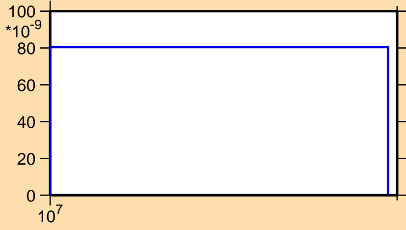
\sigma vs. E for ^{80}\text{Ge}(n,n\alpha)
