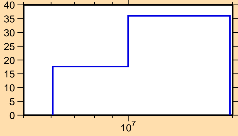
\Delta\sigma/\sigma vs. E for ^{80}\text{Ge}(n,n\text{cont.})
