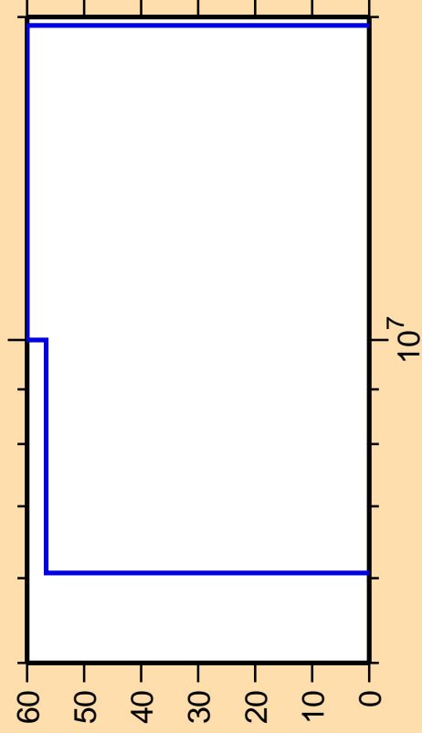
\Delta\sigma/\sigma vs. E for ^{80}\text{Ge}(n,\alpha)
