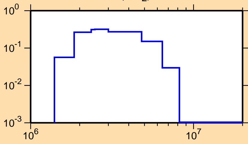
\sigma vs. E for ^{80}\text{Ge}(n,n_2)
