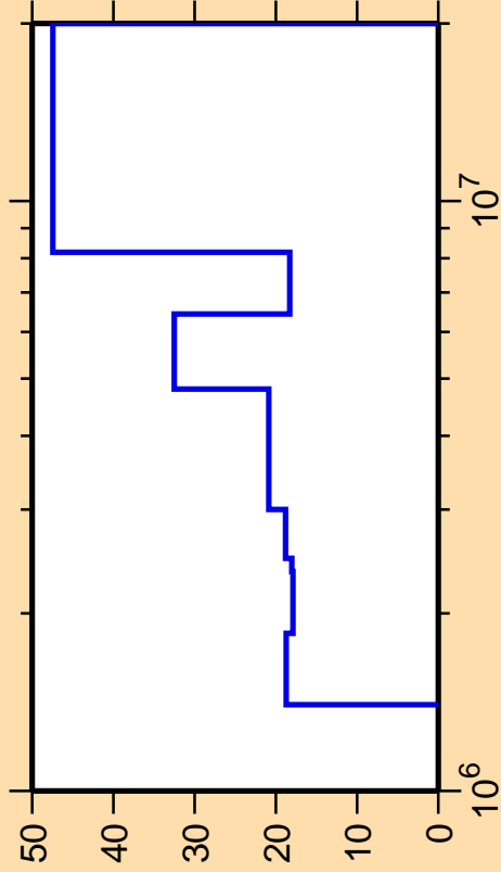
\Delta\sigma/\sigma vs. E for ^{80}\text{Ge}(n,n_2)
