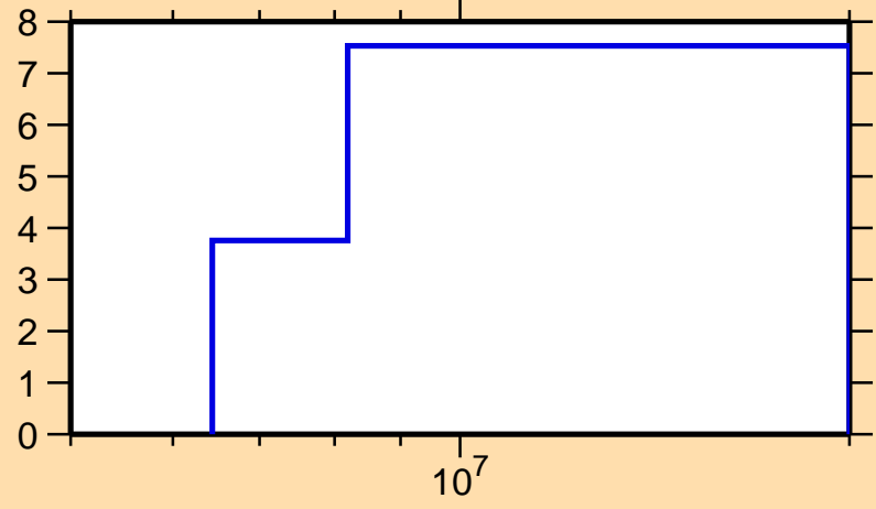
\Delta\sigma/\sigma vs. E for ^{80}\text{Ge}(n,\text{tot.})
