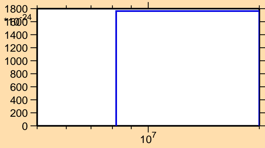
\sigma vs. E for ^{80}\text{Ge}(n,nd)
