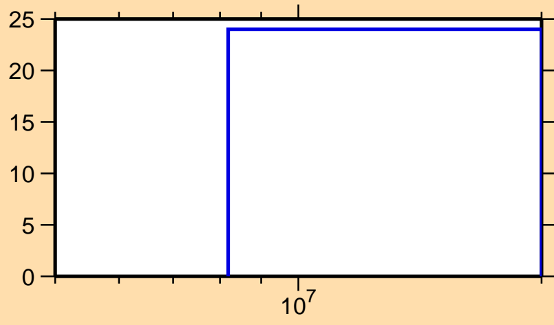
\Delta\sigma/\sigma vs. E for ^{80}\text{Ge}(n,ncont.)
