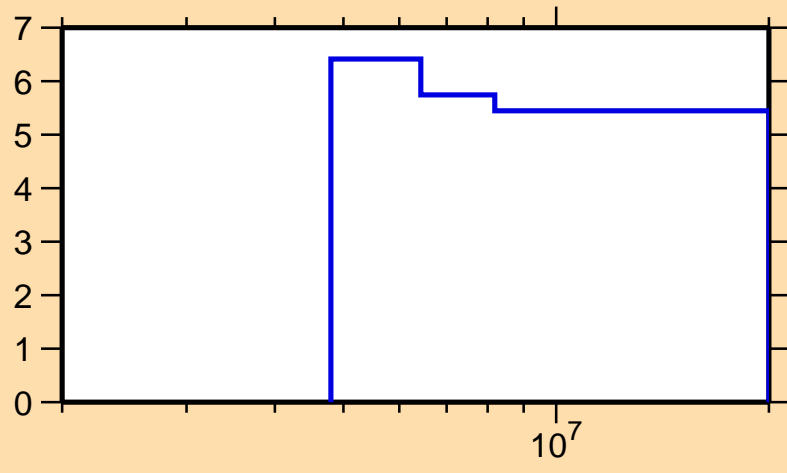
\Delta\sigma/\sigma vs. E for ^{80}\text{Ge}(n,n\text{nonel.})
