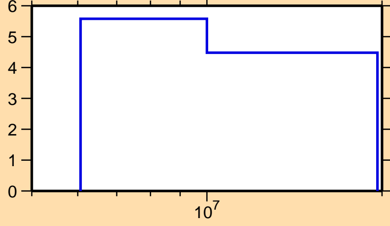
\Delta\sigma/\sigma vs. E for ^{81}\text{Ge}(n,\text{nonel.})
