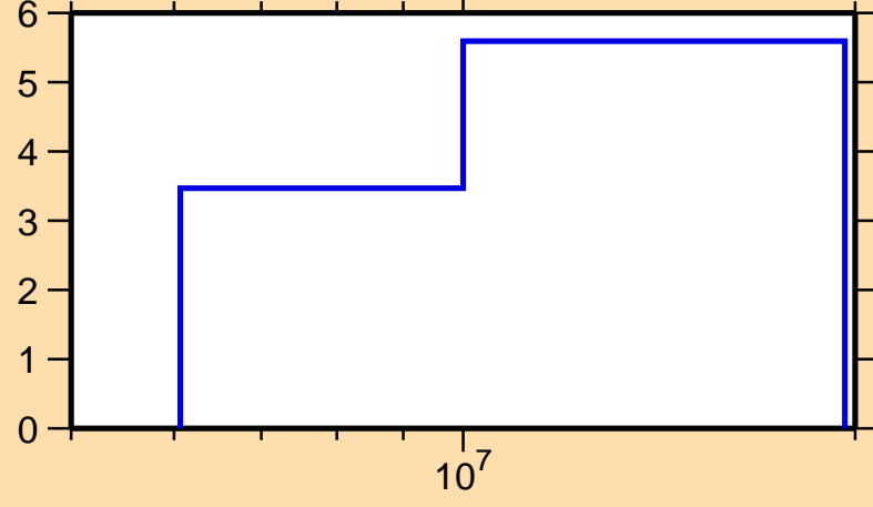
\Delta\sigma/\sigma vs. E for ^{81}\text{Ge}(n,\text{tot.})
