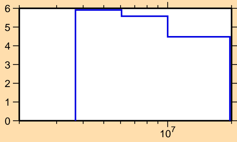
\Delta\sigma/\sigma vs. E for ^{81}\text{Ge}(n,n\text{inel.})
