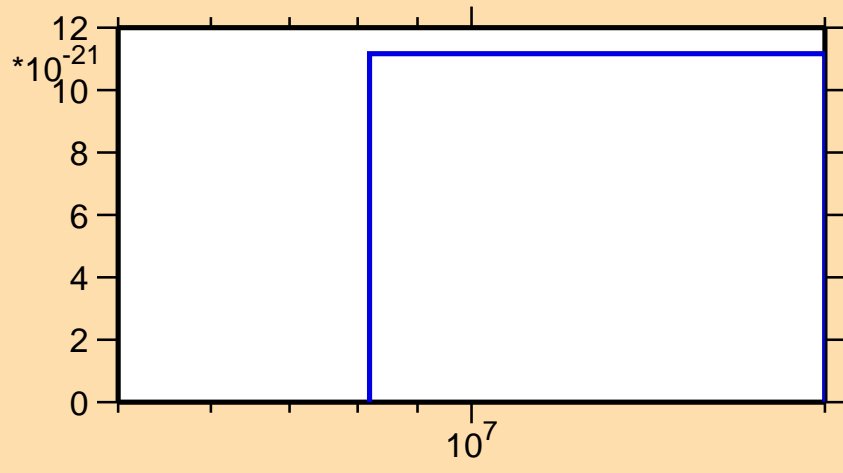
\sigma vs. E for ^{81}\text{Ge}(n,2np)
