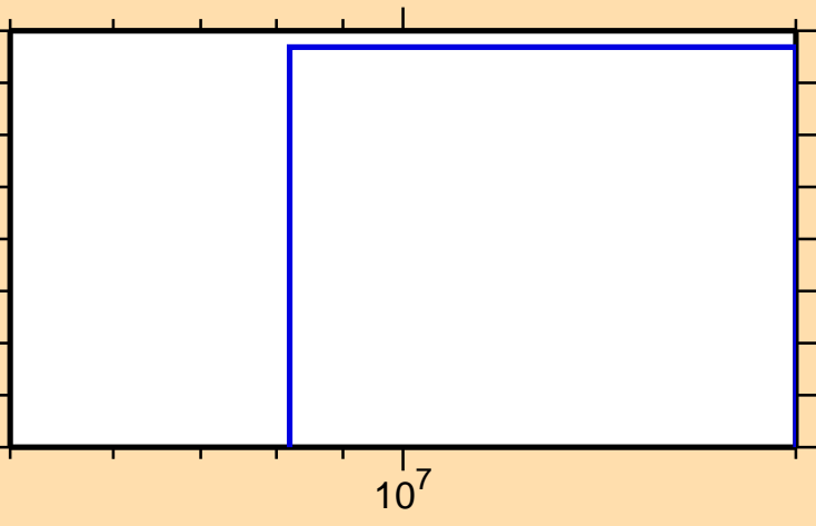
\sigma vs. E for ^{81}\text{Ge}(n,2np)
