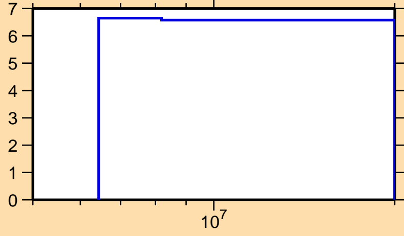
\Delta\sigma/\sigma vs. E for ^{81}\text{Ge}(n,2n)
