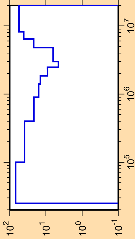
\Delta\sigma/\sigma vs. E for ^{81}\text{Ge}(n,\text{inel.})
