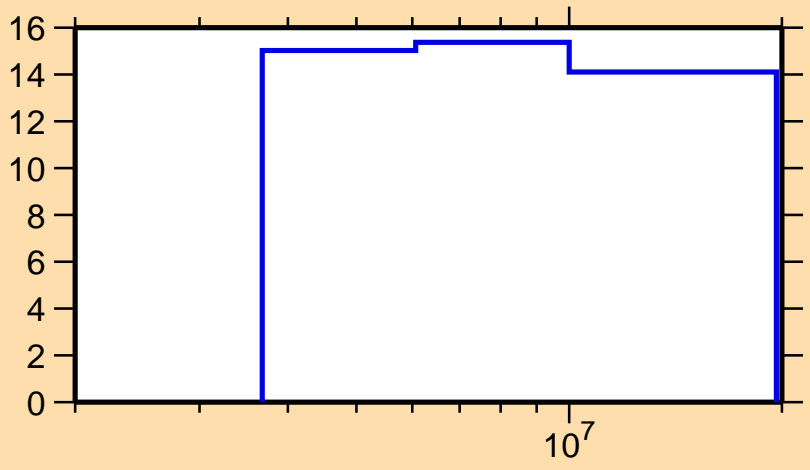
\Delta\sigma/\sigma vs. E for ^{82}\text{Ge}(n,n\text{nonel.})
