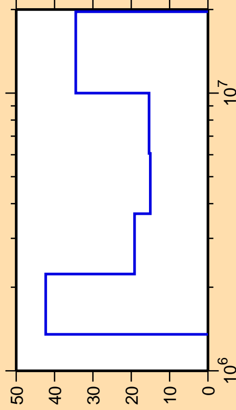
\Delta\sigma/\sigma vs. E for ^{82}\text{Ge}(n,\text{inel.})
