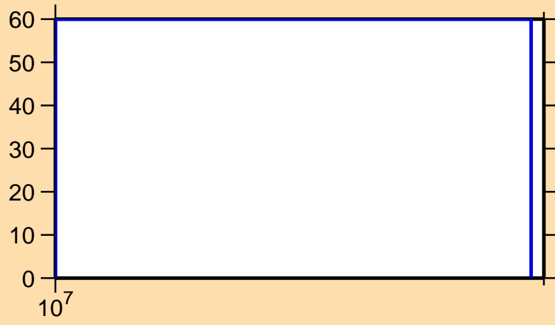
\Delta\sigma/\sigma vs. E for ^{82}\text{Ge}(n,p)
