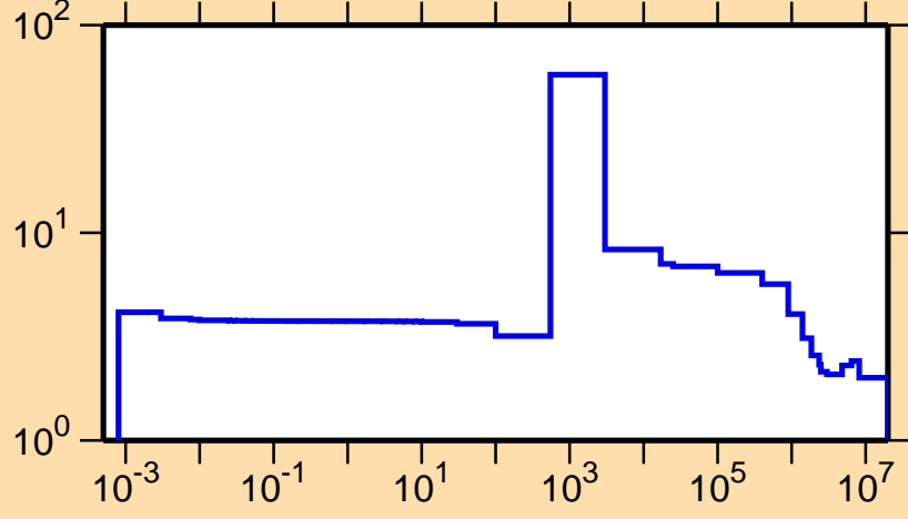
\sigma vs. E for ^{82}\text{Ge}(n,\text{el.})
