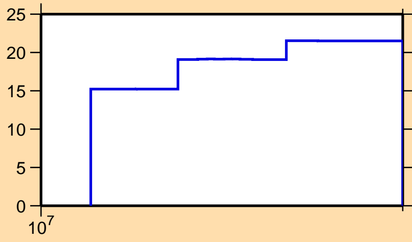
\Delta\sigma/\sigma vs. E for ^{83}\text{Ge}(n,\text{el.})
