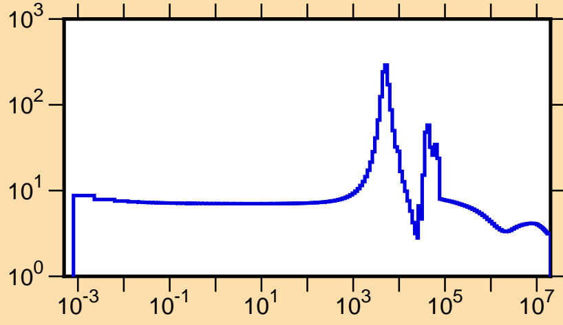
\sigma vs. E for ^{83}\text{Ge}(n,\text{tot.})
