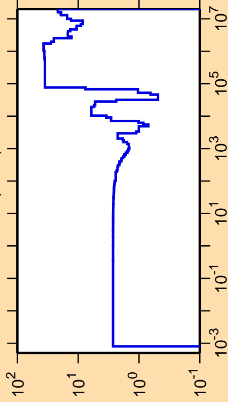
\Delta\sigma/\sigma vs. E for ^{83}\text{Ge}(n,\text{el.})
