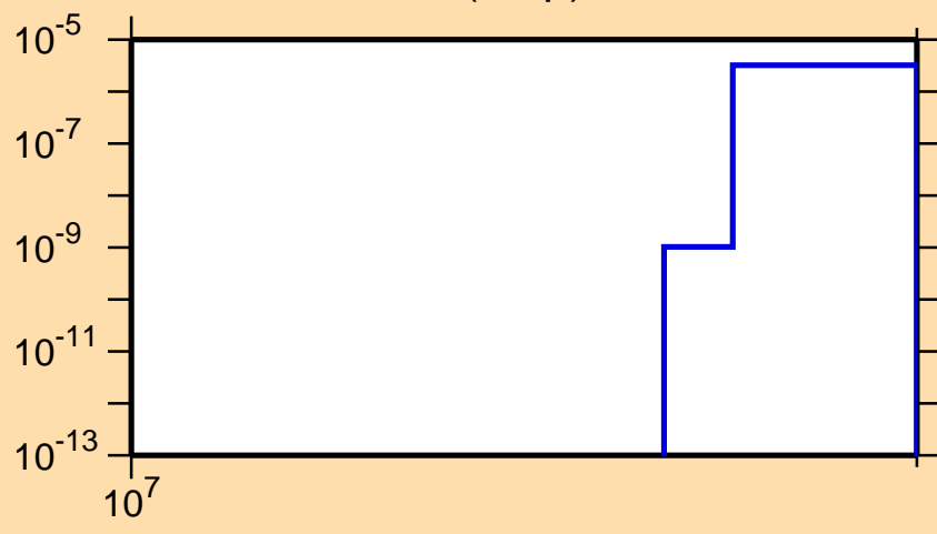
\sigma vs. E for ^{83}\text{Ge}(n,np)
