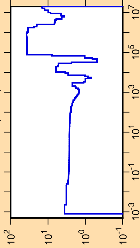
\Delta\sigma/\sigma vs. E for ^{83}\text{Ge}(n,\text{tot.})
