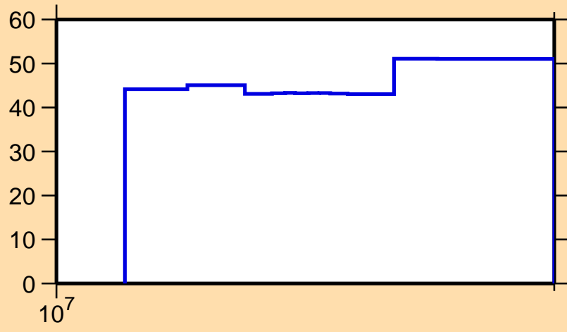
\Delta\sigma/\sigma vs. E for ^{83}\text{Ge}(n,n_1)
