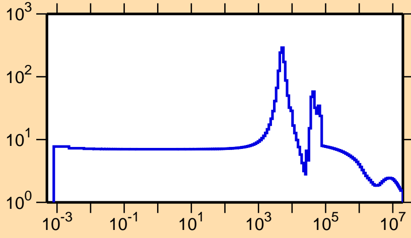
\sigma vs. E for ^{83}\text{Ge}(n,\text{el.})
