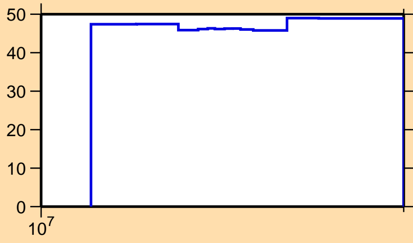
\Delta\sigma/\sigma vs. E for ^{83}\text{Ge}(n,\text{inel.})
