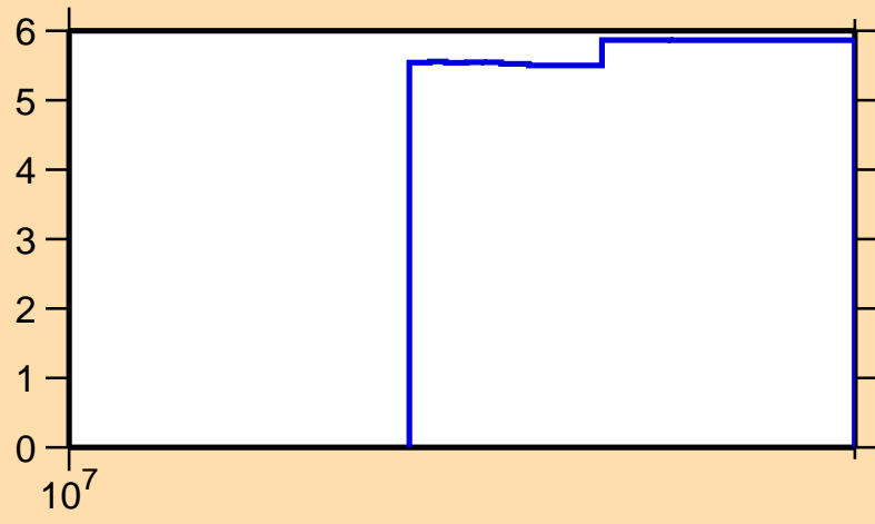
\Delta\sigma/\sigma vs. E for ^{154}\text{Hf}(n,\text{tot.})
