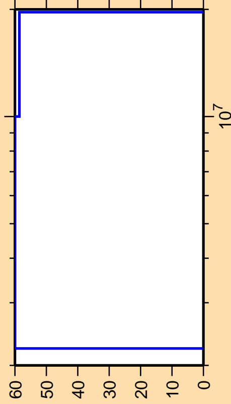
\Delta\sigma/\sigma vs. E for ^{154}\text{Hf}(n,n_4)
