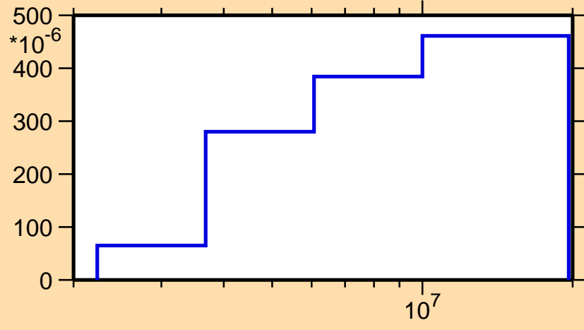
\sigma vs. E for ^{154}\text{Hf}(n,n_4)
