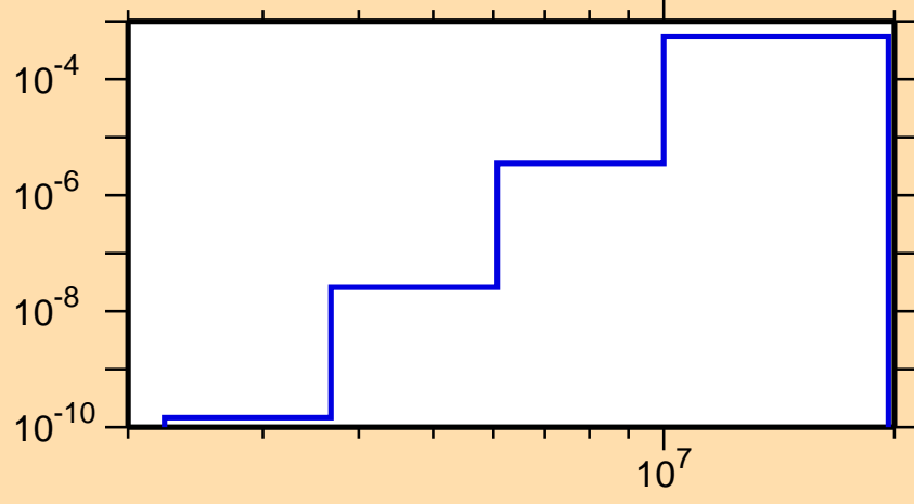
\sigma vs. E for ^{154}\text{Hf}(n,n\alpha)
