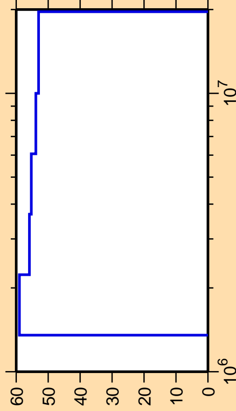
\Delta\sigma/\sigma vs. E for ^{154}\text{Hf}(n,n_2)
