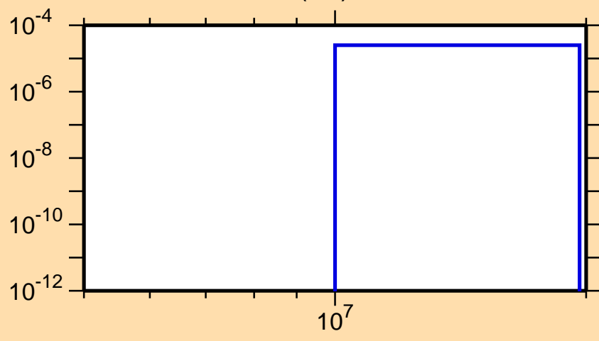
\sigma vs. E for ^{154}\text{Hf}(n,t)
