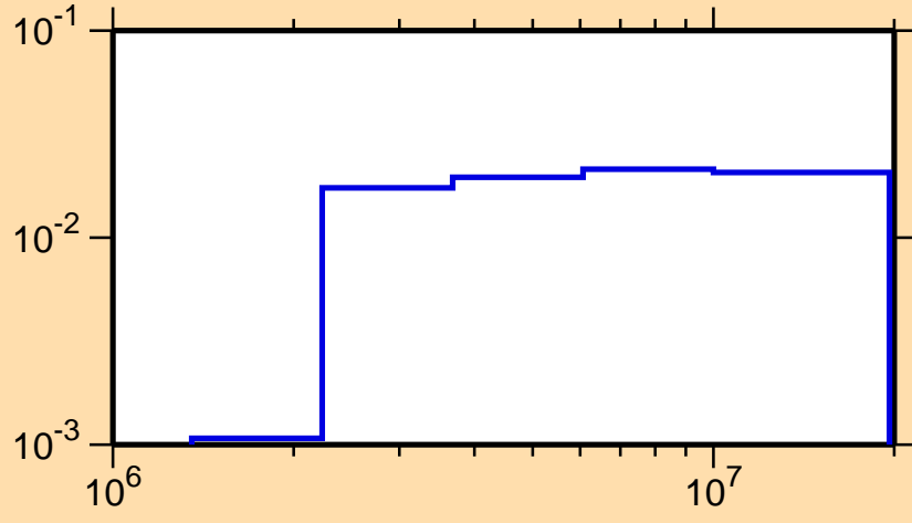
\sigma vs. E for ^{154}\text{Hf}(n,n_2)
