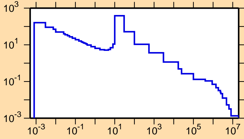
\sigma vs. E for ^{154}\text{Hf}(n,\gamma)
