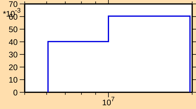
\sigma vs. E for ^{159}\text{Hf}(n,n\text{cont.})
