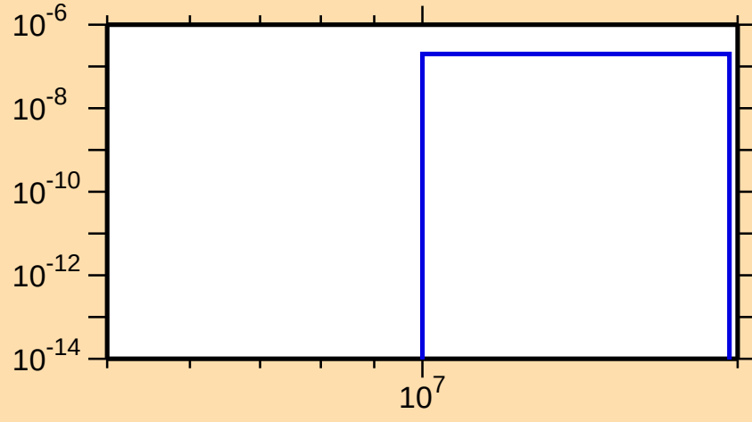
\sigma vs. E for ^{159}\text{Hf}(n,\text{nd})
