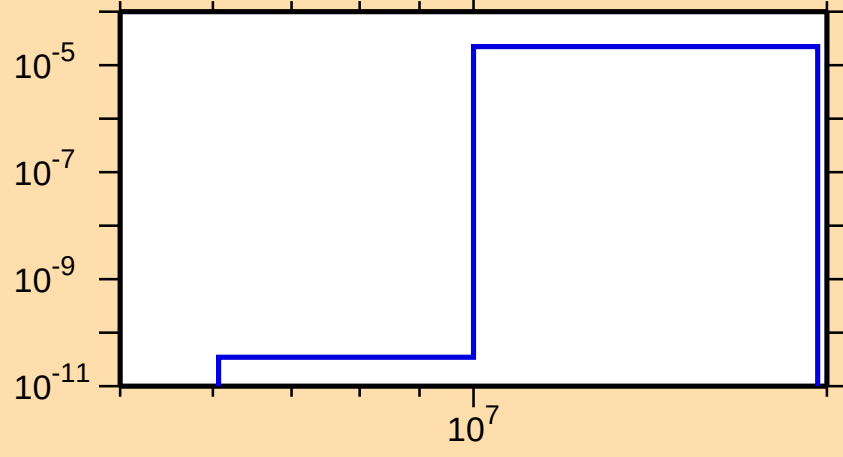
\sigma vs. E for ^{159}\text{Hf}(\text{mt } 45)
