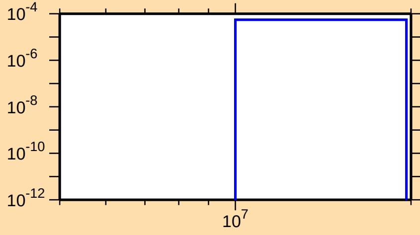
\sigma vs. E for ^{159}\text{Hf}(n,2n\alpha)
