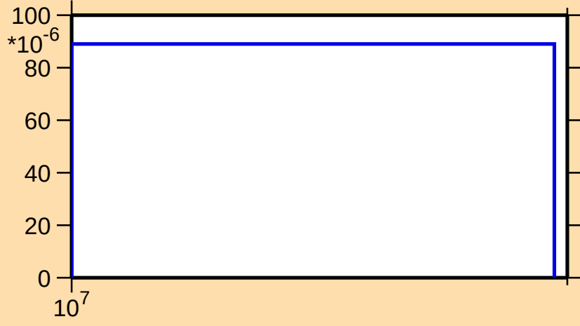
\sigma vs. E for ^{159}\text{Hf}(n,2np)
