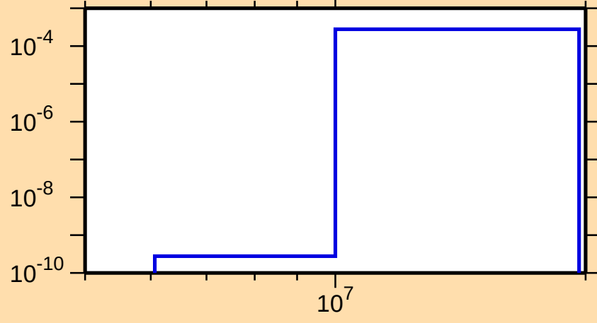
\sigma vs. E for ^{159}\text{Hf}(n,t)
