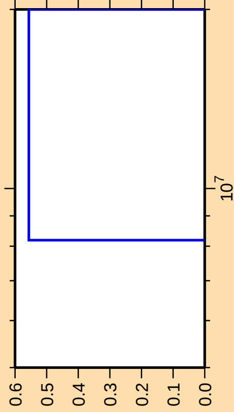
\Delta\sigma/\sigma vs. E for ^{159}\text{Hf}(n,nt)
