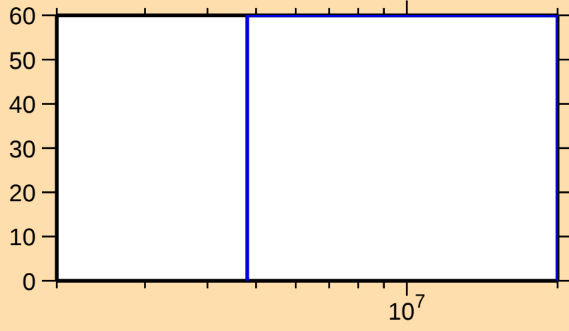
\Delta\sigma/\sigma vs. E for ^{159}\text{Hf}(n,n_1)
