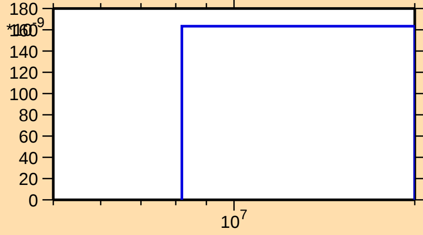
\sigma vs. E for ^{159}\text{Hf}(n,\text{nd})
