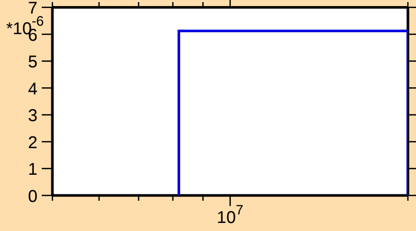
\sigma vs. E for ^{159}\text{Hf}(n,\text{pd})
