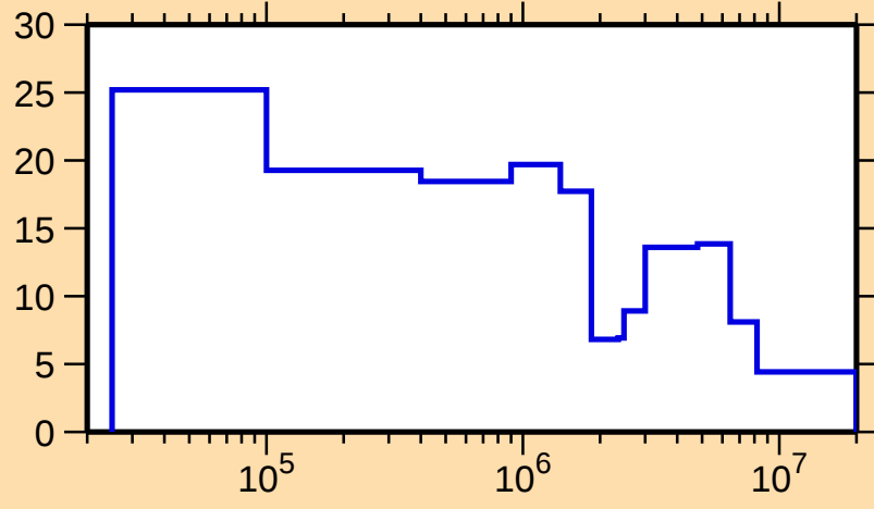
\Delta\sigma/\sigma vs. E for ^{159}\text{Hf}(n,\text{tot.})
