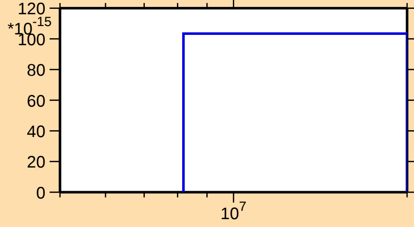
\sigma vs. E for ^{159}\text{Hf}(n,nt)
