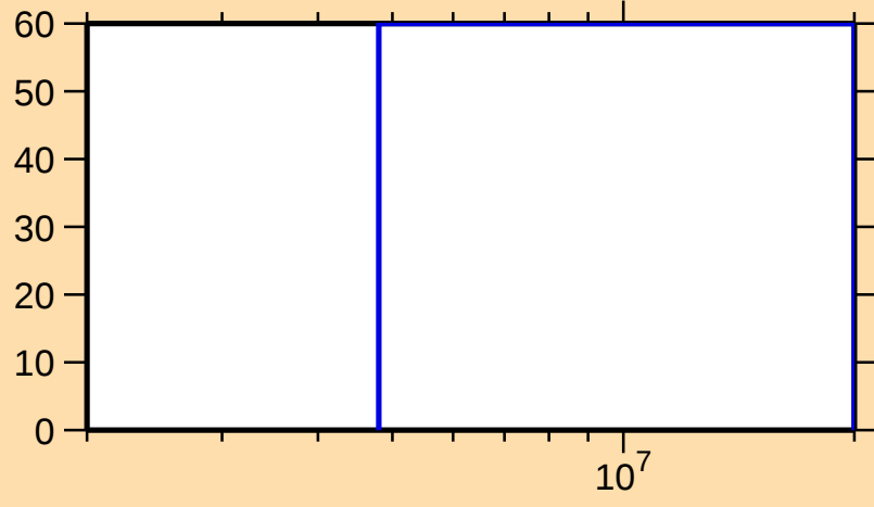
\Delta\sigma/\sigma vs. E for ^{159}\text{Hf}(n,n\text{cont.})
