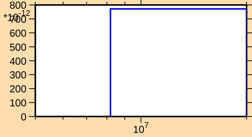
\sigma vs. E for ^{159}\text{Hf}(\text{mt } 34)
