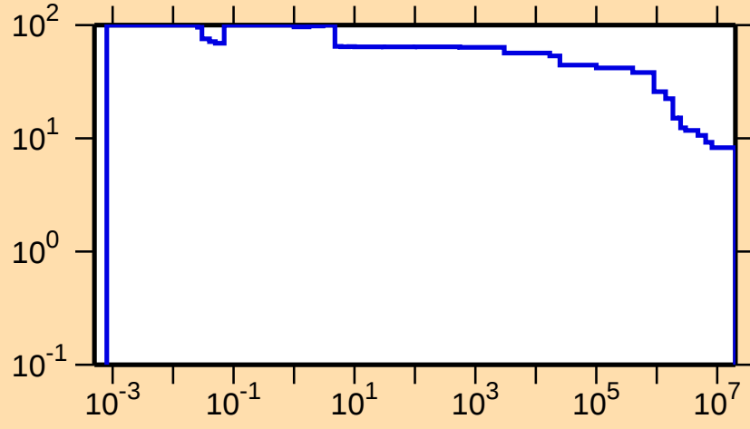
\Delta\sigma/\sigma vs. E for ^{159}\text{Hf}(n,\text{nonel.})
