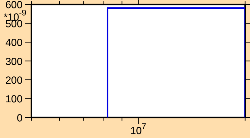
\sigma vs. E for ^{159}\text{Hf}(n,\text{pt})
