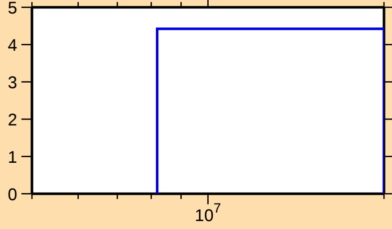
\Delta\sigma/\sigma vs. E for ^{159}\text{Hf}(n,\text{tot.})
