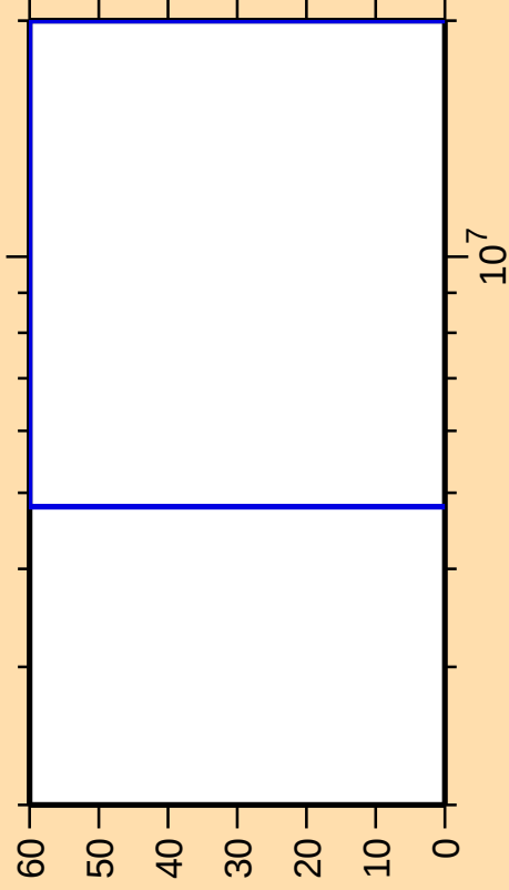
\Delta\sigma/\sigma vs. E for ^{159}\text{Hf}(n,\text{ncont.})
