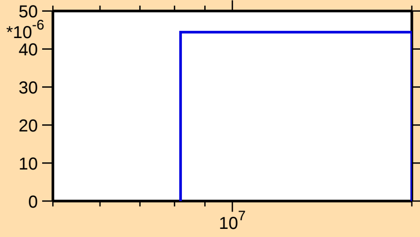
\sigma vs. E for ^{159}\text{Hf}(n,2n\alpha)
