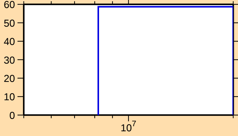
\Delta\sigma/\sigma vs. E for ^{159}\text{Hf}(n,\text{inel.})
