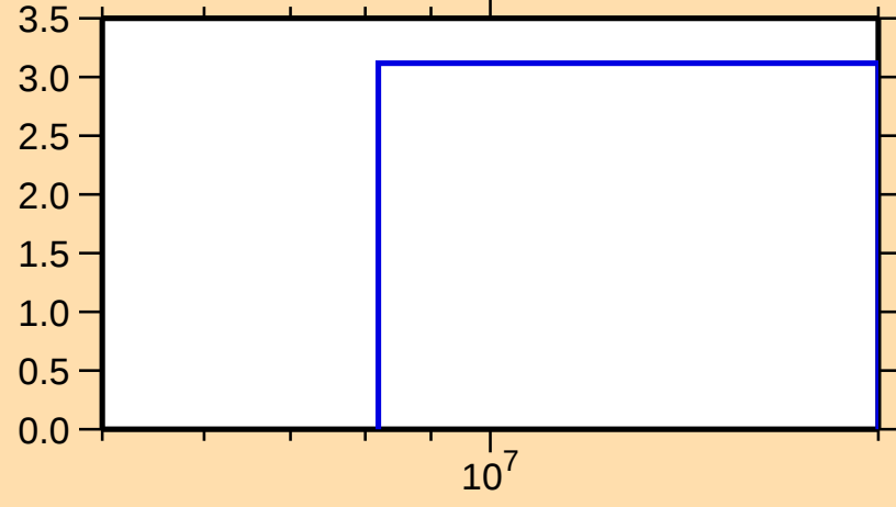
\Delta\sigma/\sigma vs. E for ^{159}\text{Hf}(n,\text{el.})
