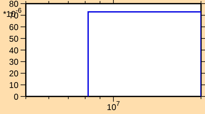
\sigma vs. E for ^{159}\text{Hf}(n,2np)
