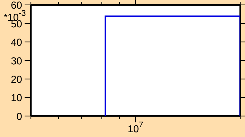
\sigma vs. E for ^{159}\text{Hf}(n,2n)
