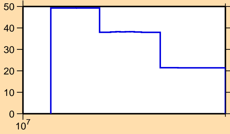
\Delta\sigma/\sigma vs. E for ^{160}\text{Hf}(n,\text{inel.})
