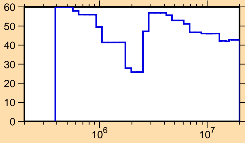
\Delta\sigma/\sigma vs. E for ^{160}\text{Hf}(n,n_1)
