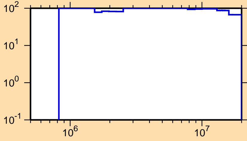
\Delta\sigma/\sigma vs. E for ^{160}\text{Hf}(n,n\text{cont.})
