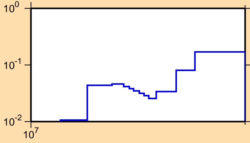
\sigma vs. E for ^{160}\text{Hf}(n,2n)
