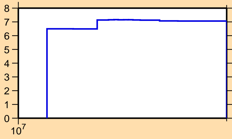
\Delta\sigma/\sigma vs. E for ^{160}\text{Hf}(n,\text{el.})
