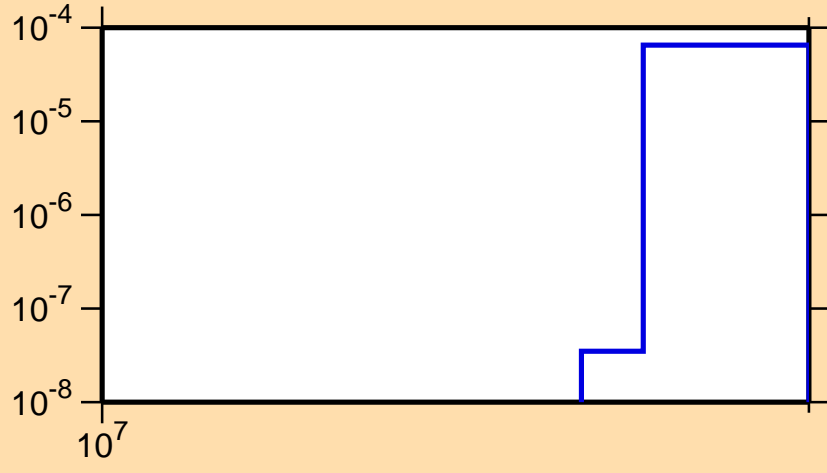
\sigma vs. E for ^{160}\text{Hf}(n,2np)
