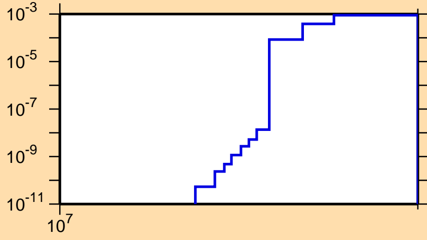
\sigma vs. E for ^{160}\text{Hf}(n,2n\alpha)
