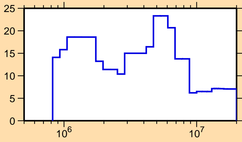
\Delta\sigma/\sigma vs. E for ^{160}\text{Hf}(n,\text{el.})
