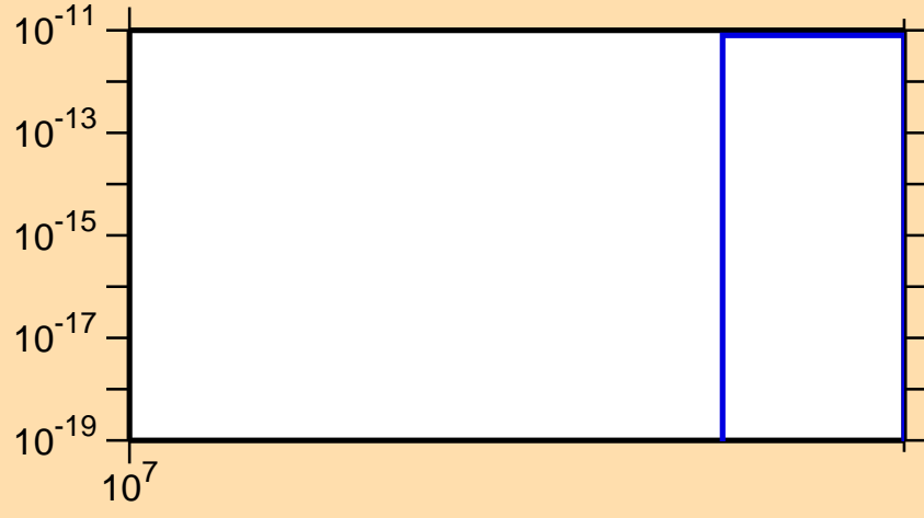
\sigma vs. E for ^{160}\text{Hf}(n,nt)
