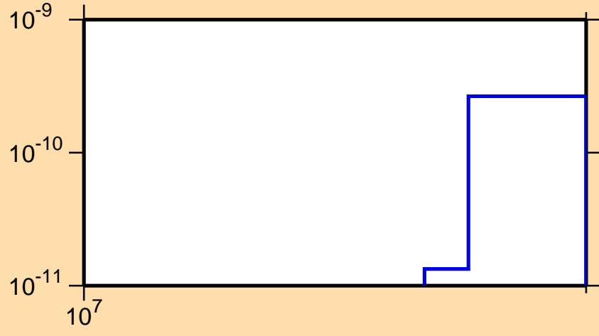
\sigma vs. E for ^{160}\text{Hf}(\text{mt } 34)
