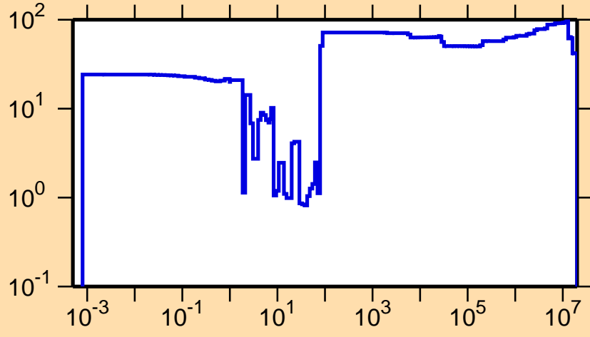
\Delta\sigma/\sigma vs. E for ^{160}\text{Hf}(n,\gamma)
