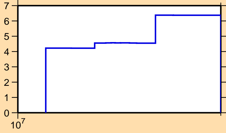
\Delta\sigma/\sigma vs. E for ^{160}\text{Hf}(n,\text{tot.})
