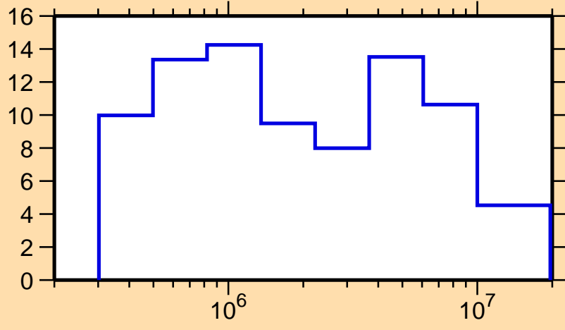
\Delta\sigma/\sigma vs. E for ^{160}\text{Hf}(n,\text{tot.})
