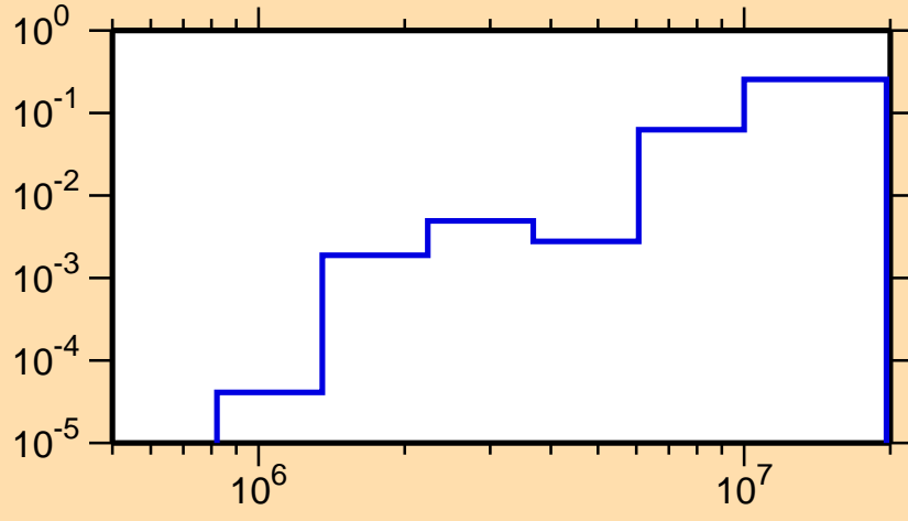
\sigma vs. E for ^{160}\text{Hf}(n,n\text{cont.})
