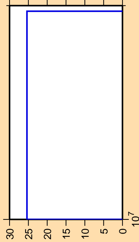
\Delta\sigma/\sigma vs. E for ^{160}\text{Hf} (mt 34)
