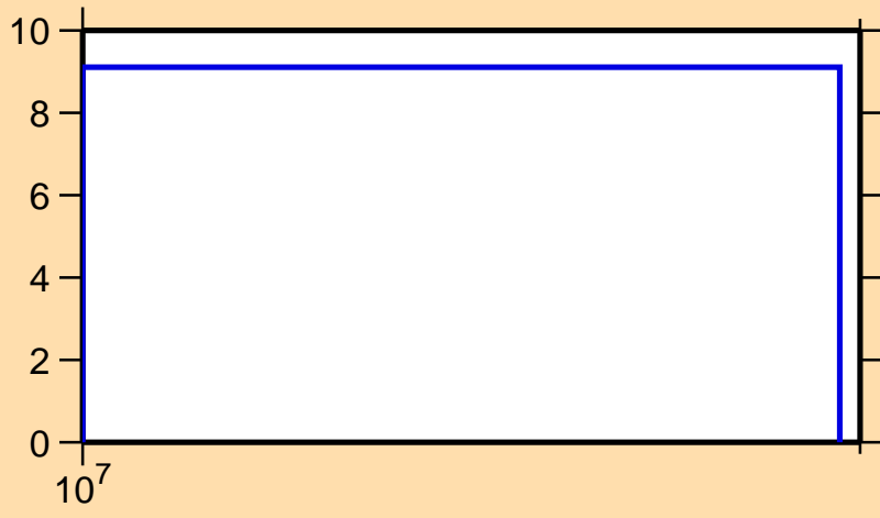
\Delta\sigma/\sigma vs. E for ^{160}\text{Hf}(n,\text{nonel.})
