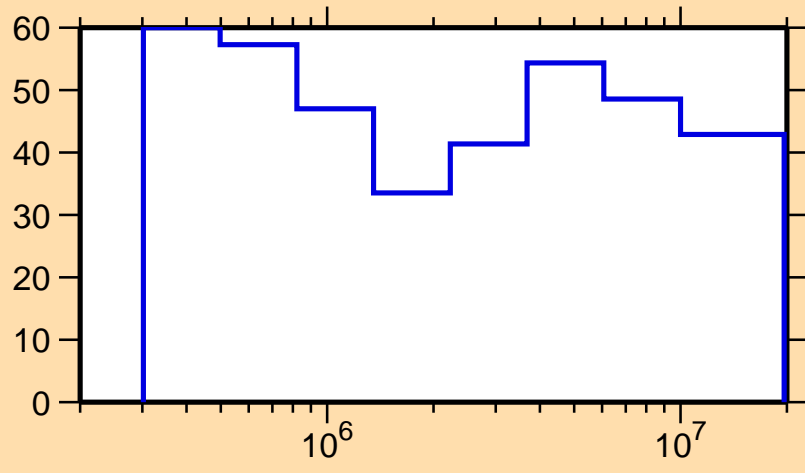
\Delta\sigma/\sigma vs. E for ^{160}\text{Hf}(n,n_1)
