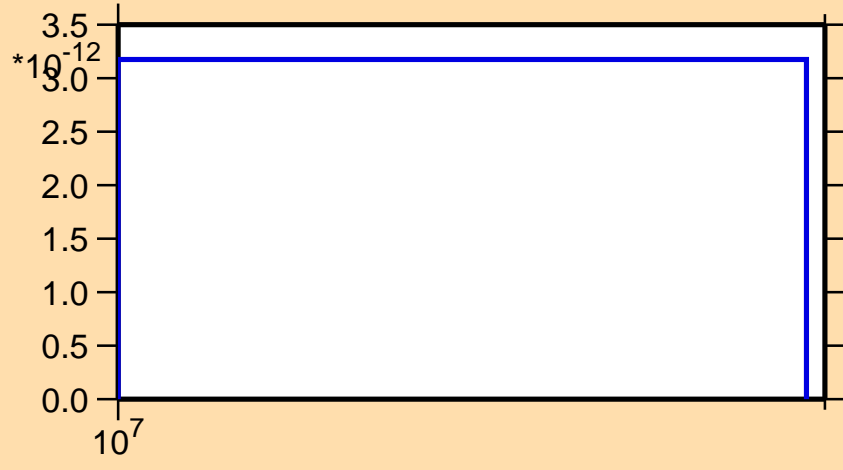
\sigma vs. E for ^{160}\text{Hf} (mt 34)
