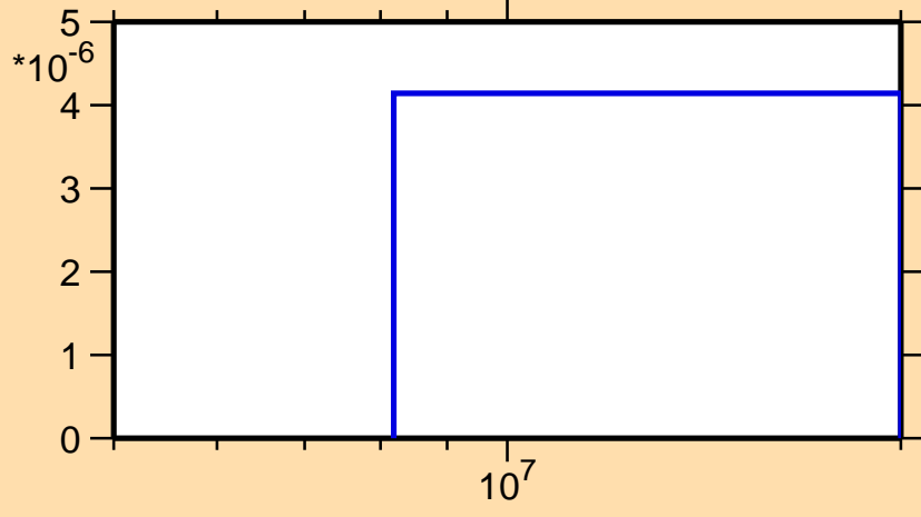
\sigma vs. E for ^{160}\text{Hf}(n,\text{pd})
