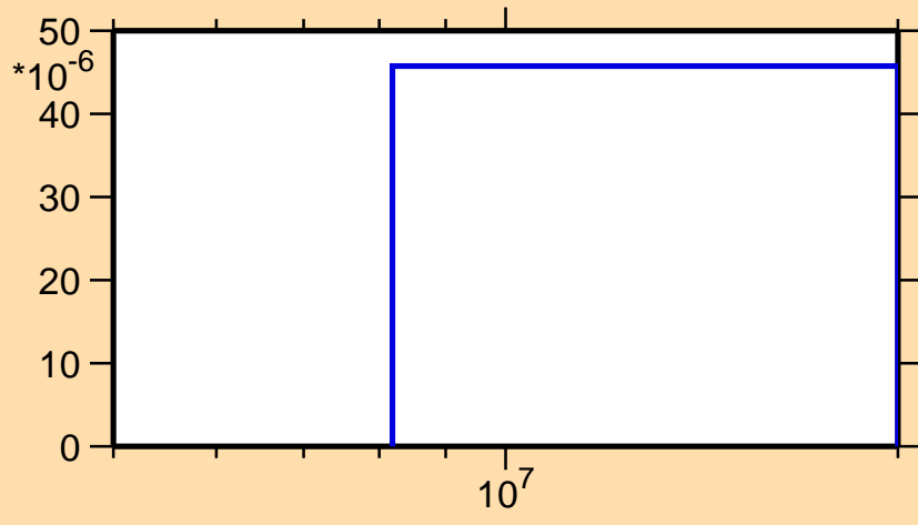
\sigma vs. E for ^{160}\text{Hf}(n,t)
