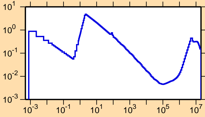
\sigma vs. E for ^{162}\text{Hf}(n,p)
