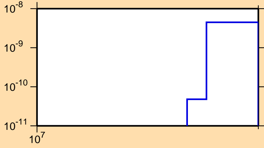
\sigma vs. E for ^{162}\text{Hf}(n,\text{pt})
