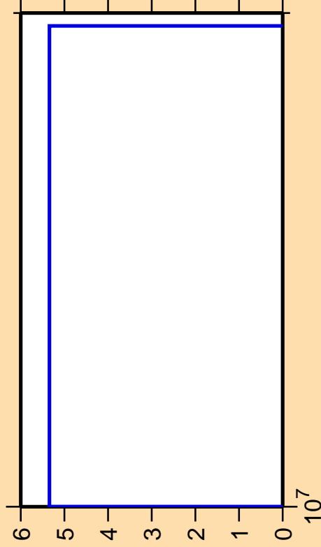
\Delta\sigma/\sigma vs. E for ^{162}\text{Hf} (mt 34)
