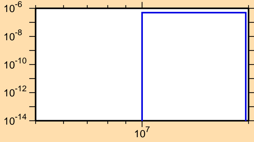
\sigma vs. E for ^{162}\text{Hf} (mt 45)
