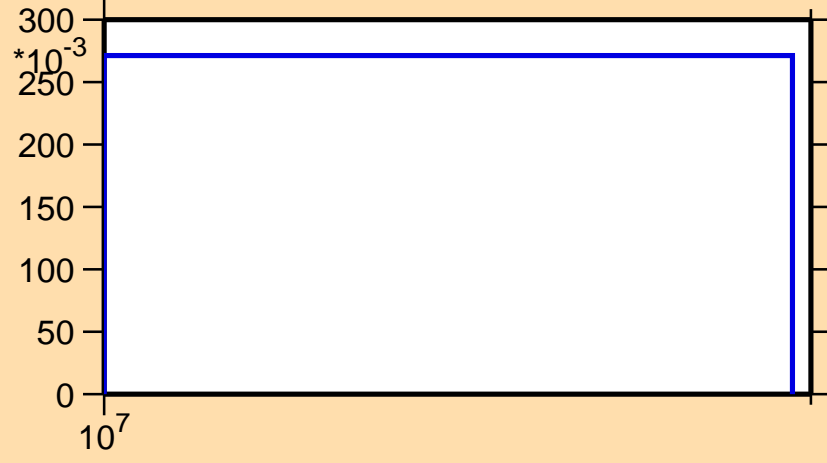
\sigma vs. E for ^{162}\text{Hf}(n,2n)
