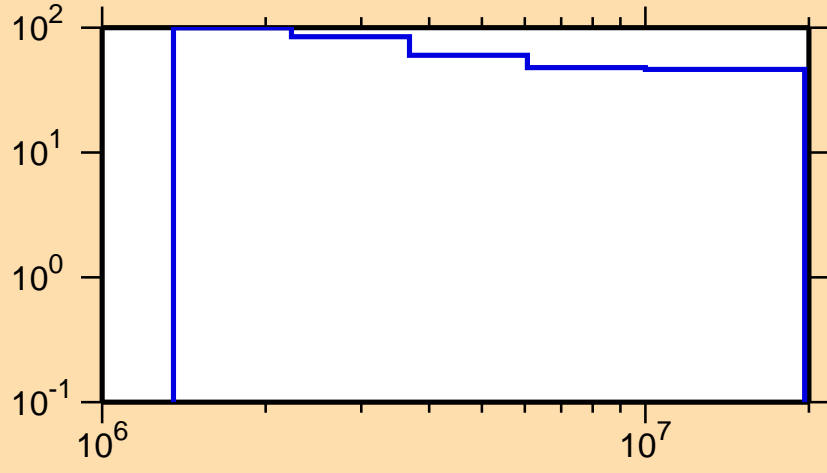
\Delta\sigma/\sigma vs. E for ^{162}\text{Hf}(n,ncont.)
