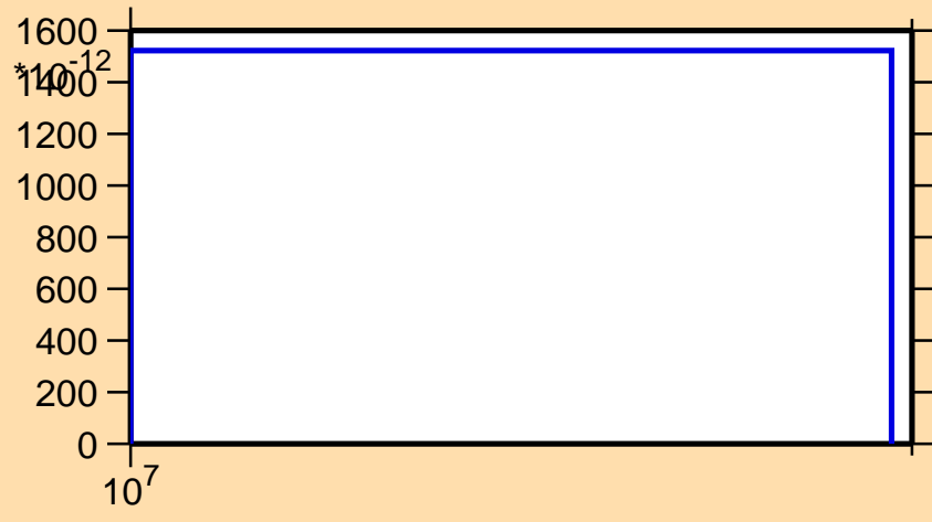
\sigma vs. E for ^{162}\text{Hf}(n,\text{nd})
