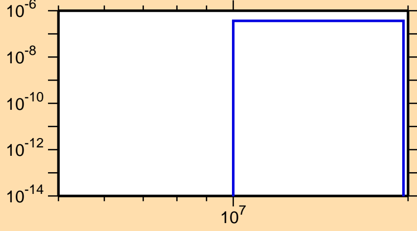
\sigma vs. E for ^{162}\text{Hf}(n,pd)
