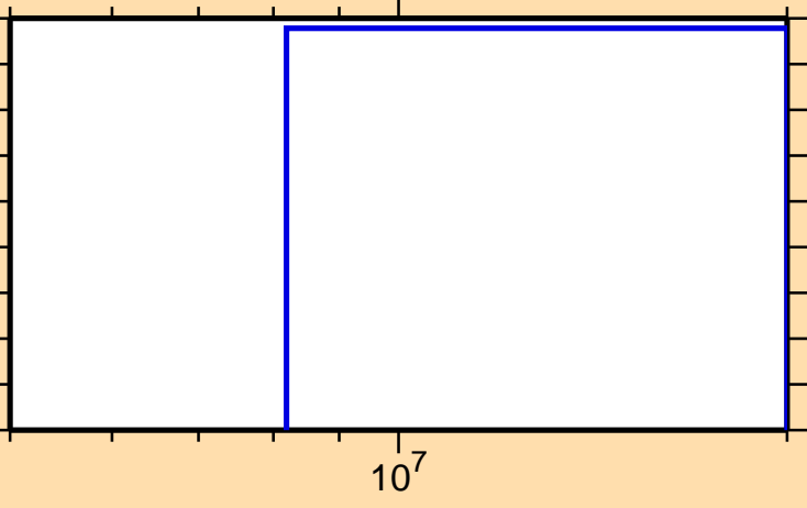
\sigma vs. E for ^{162}\text{Hf}(n,2n\alpha)
