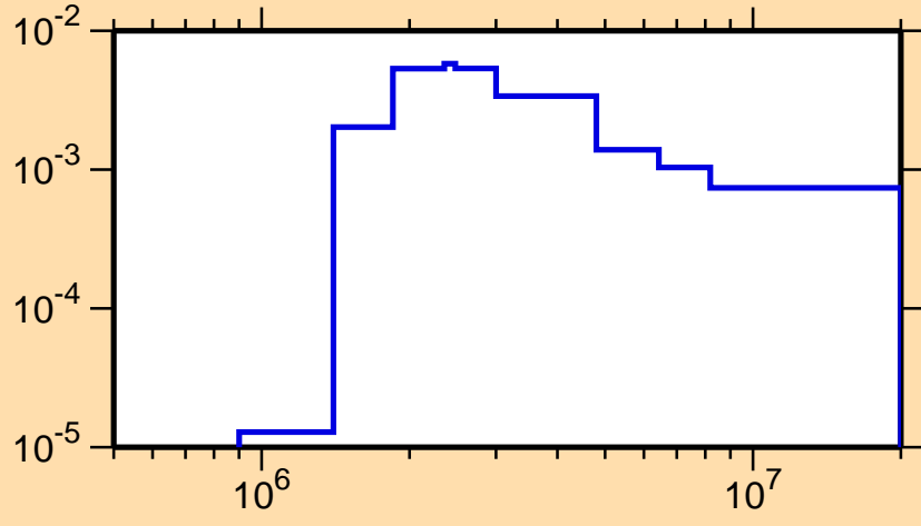
\sigma vs. E for ^{162}\text{Hf}(n,n_3)
