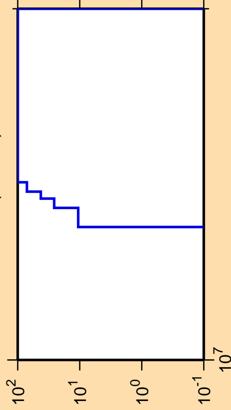
\Delta\sigma/\sigma vs. E for ^{164}\text{Hf(mt117)}
