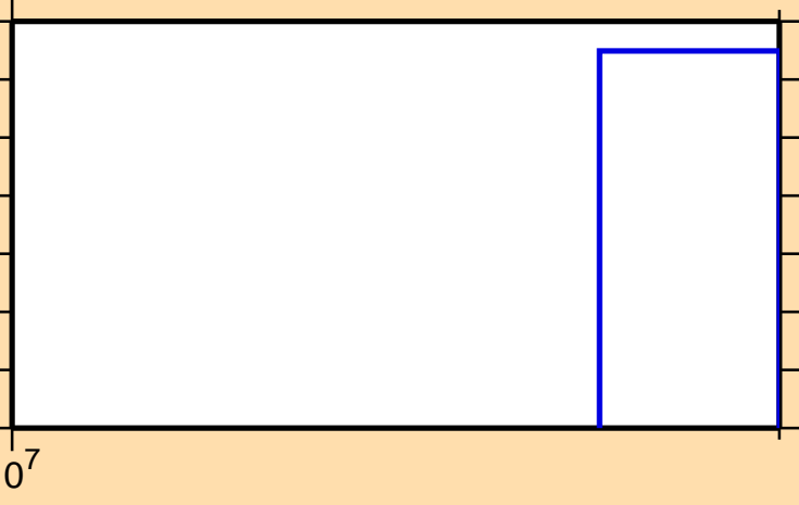
\sigma vs. E for ^{164}\text{Hf}(n,3n)
