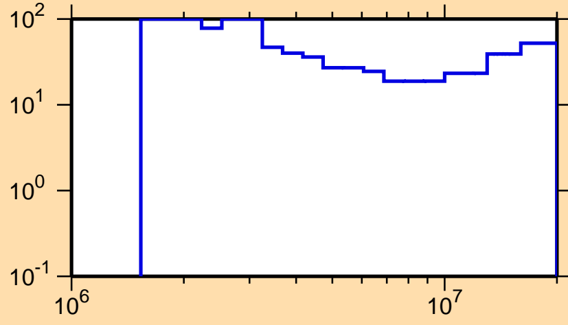
\Delta\sigma/\sigma vs. E for ^{164}\text{Hf}(n,n\text{cont.})
