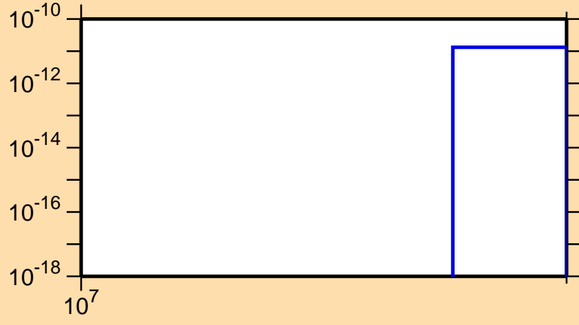
\sigma vs. E for ^{164}\text{Hf}(n,nt)
