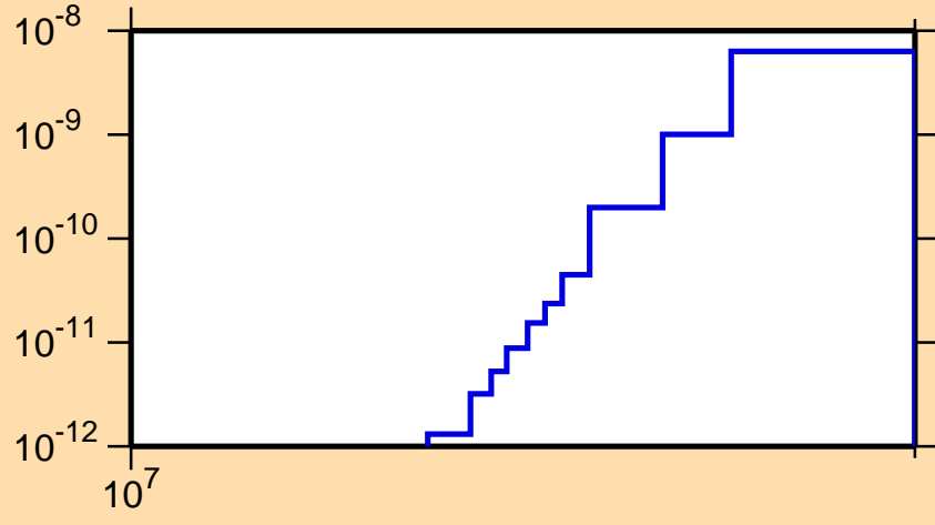
\sigma vs. E for ^{164}\text{Hf(mt117)}
