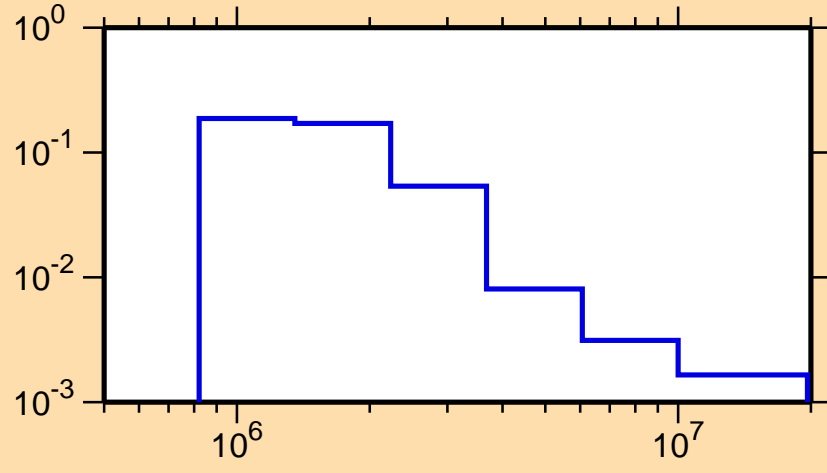
\sigma vs. E for ^{164}\text{Hf}(n,n_4)
