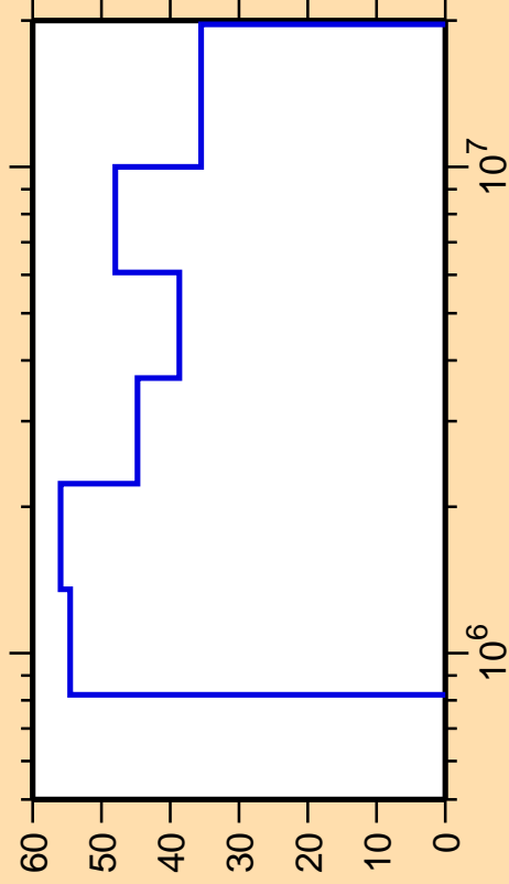
\Delta\sigma/\sigma vs. E for ^{164}\text{Hf}(n,n_4)
