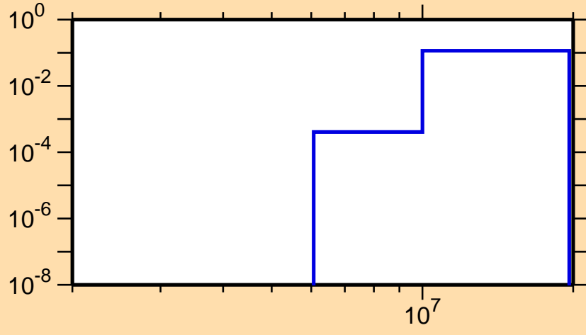
\sigma vs. E for ^{164}\text{Hf}(n,np)
